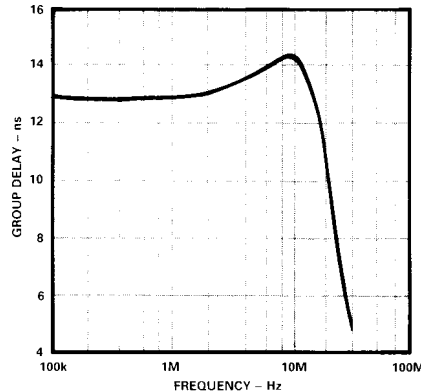
Figure 31. Group Delay Characteristics of Undifferentiated Output
