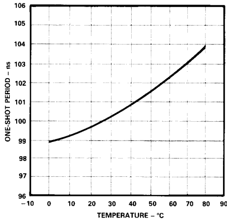
Figure 14. One-Shot Period vs. Temperature ( R_{\text{SET}} = 30\text{ k}\Omega )
