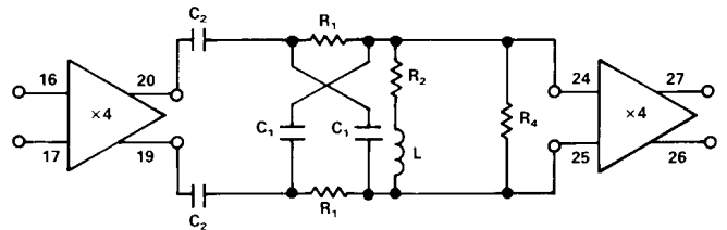
Figure 21. RLC Equalizer
