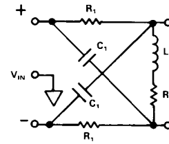
Figure 25. RLC Lattice
