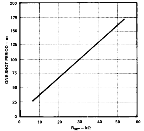
Figure 15. One-Shot Period vs. R_{\text{SET}}
