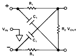
Figure 24. RC Lattice
