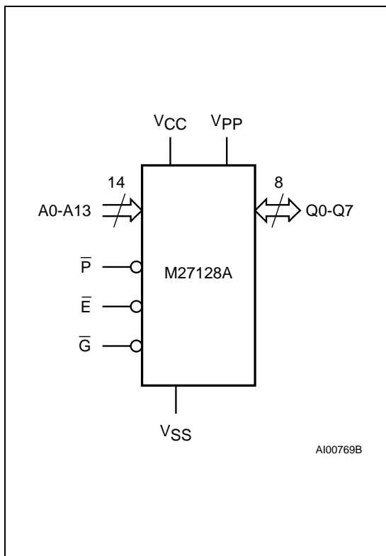
Figure 1. Logic Diagram
