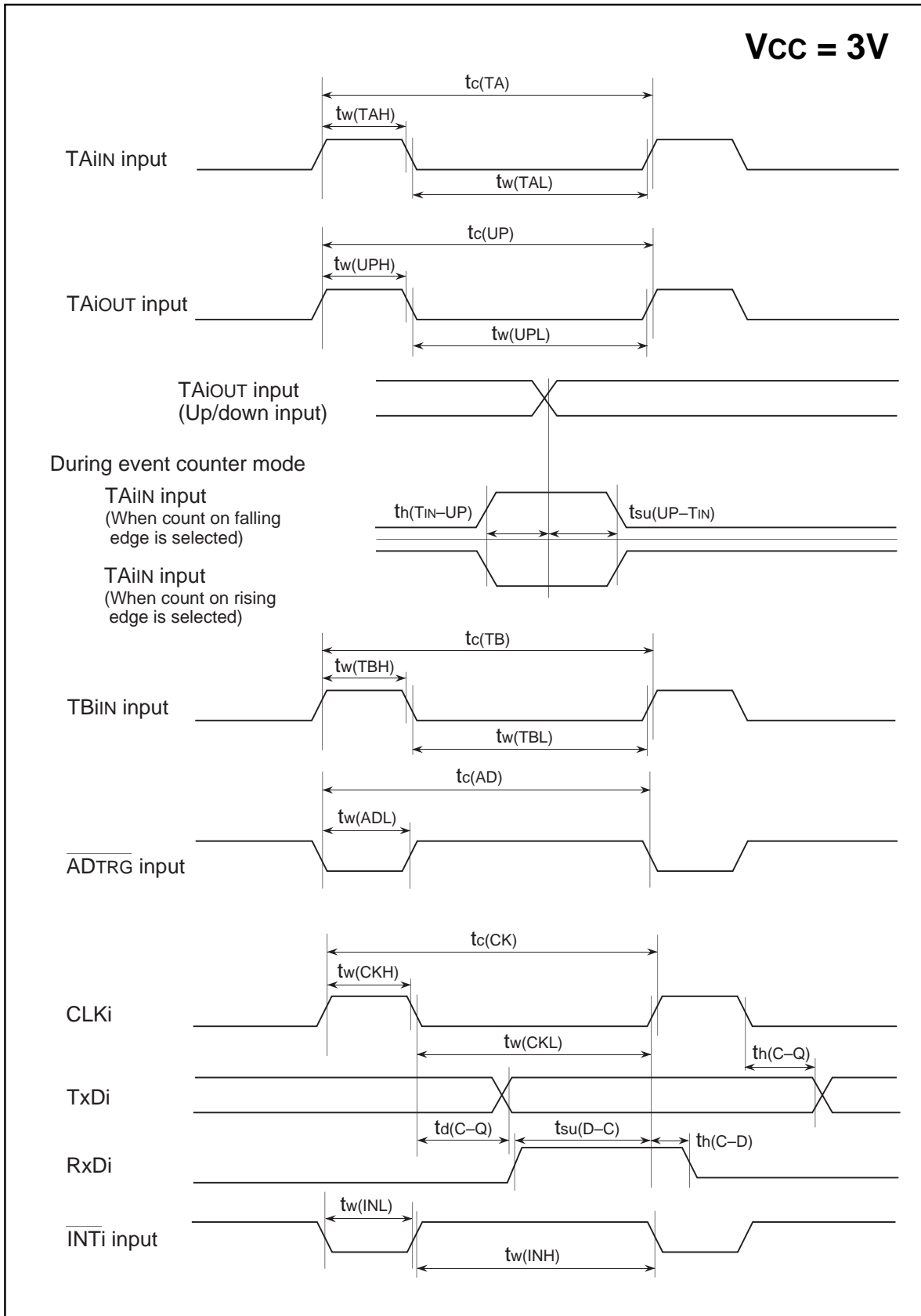
Figure 1.20.2. V_{CC}=3V timing diagram
