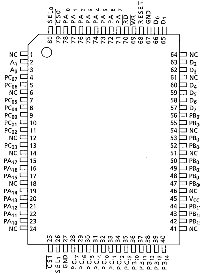
TMP82C265BF-2/TMP82C265BF-10
