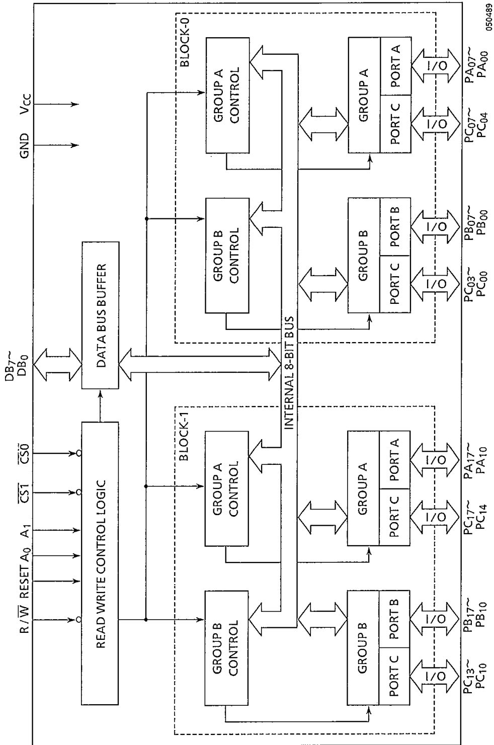
TMP82C255A
