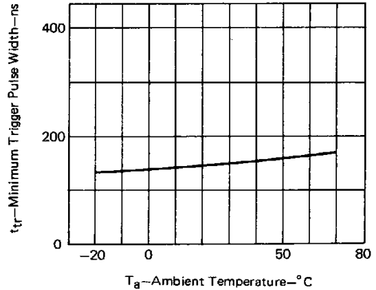
MINIMUM TRIGGER PULSE WIDTH
