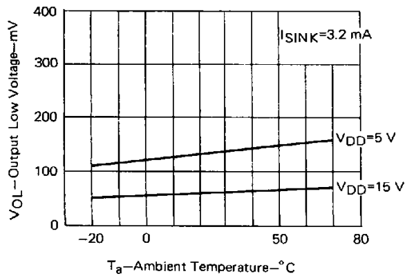
OUTPUT LOW VOLTAGE
