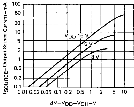
OUTPUT SOURCE CURRENT
