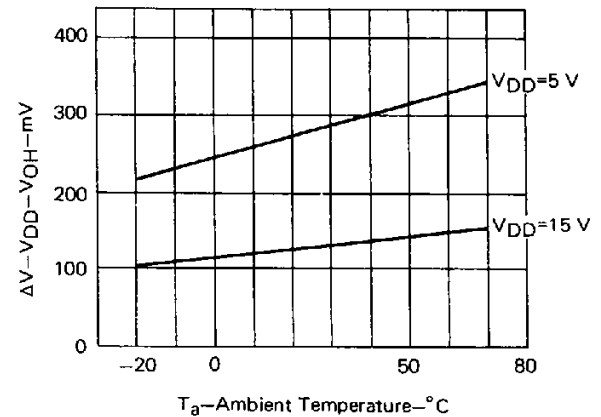
V DD -OUTPUT HIGH VOLTAGE
