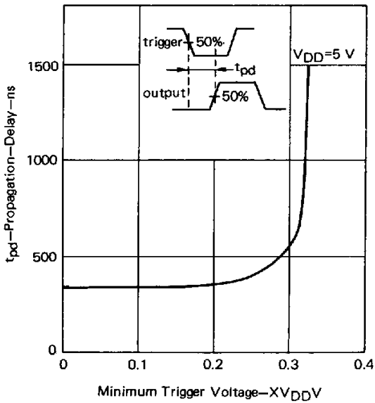
PROPAGATION DELAY
