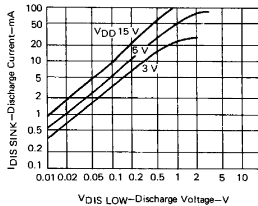
DISCHARGE CURRENT
