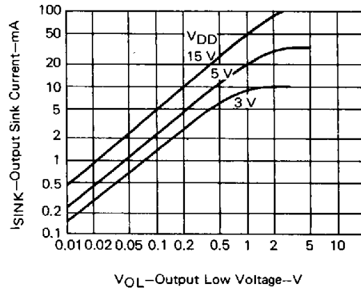
OUTPUT SINK CURRENT
