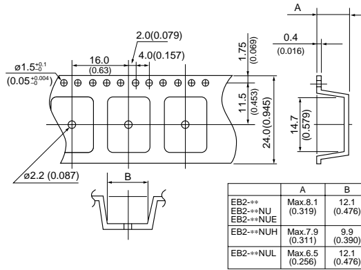
Tape Dimensions Unit : mm (inch)
