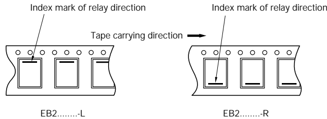
Relay orientation mark and tape carrying direction.
