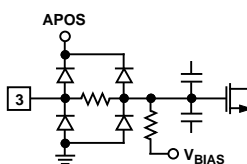
Circuit A
