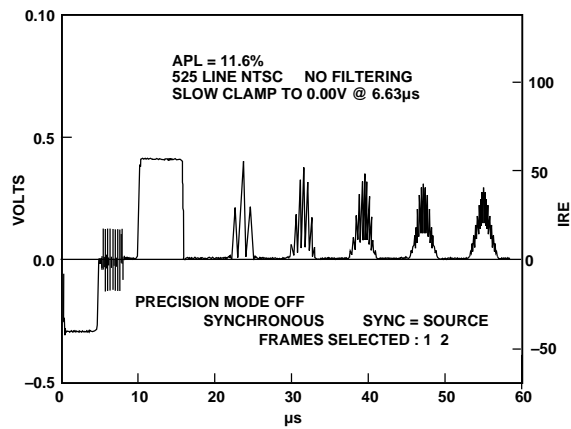
Figure 8. Multipulse, NTSC
