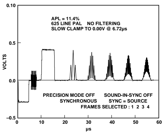
Figure 9. Multipulse, PAL
