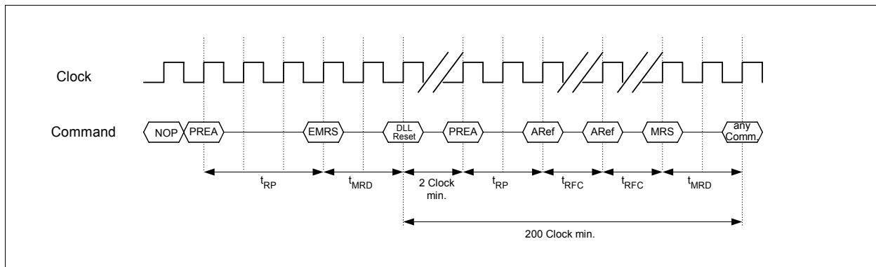
Figure 9 Power-Up Sequence
