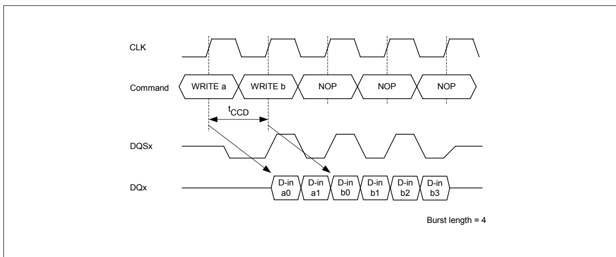
Figure 27 Write interrupted by Write
