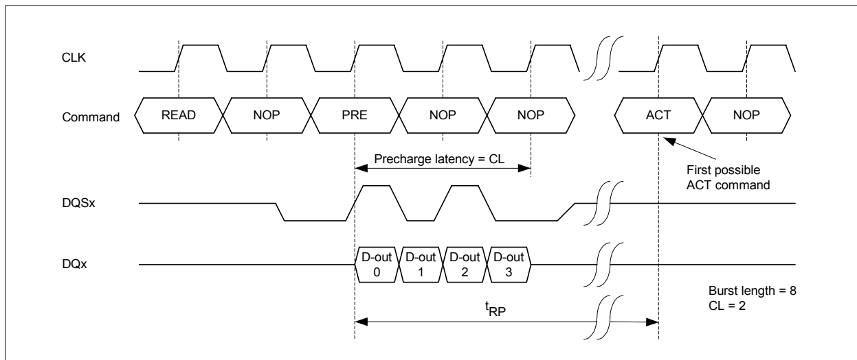
Figure 26 Read interrupted by Precharge
