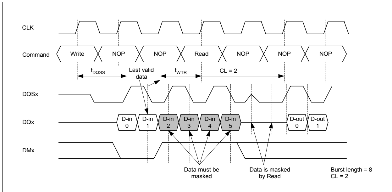
Figure 28 Write interrupted by Read
