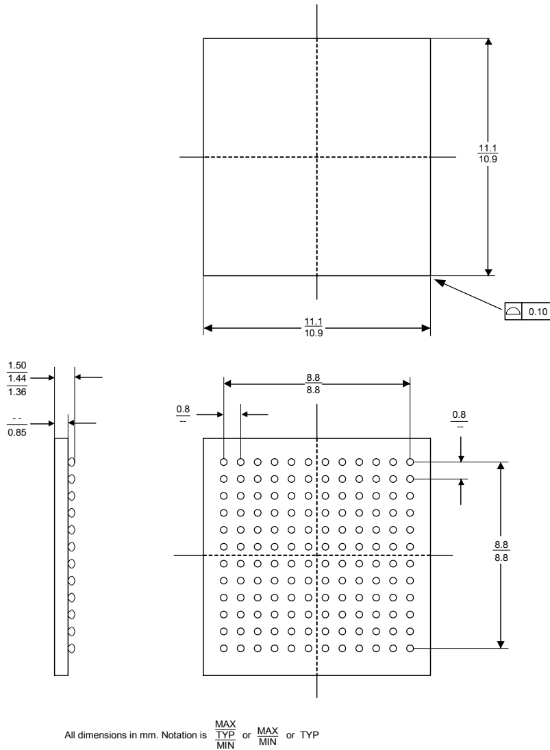
Figure 32 Package Outlines
