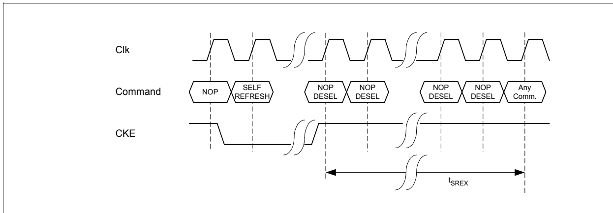
Figure 14 Self Refresh timing
