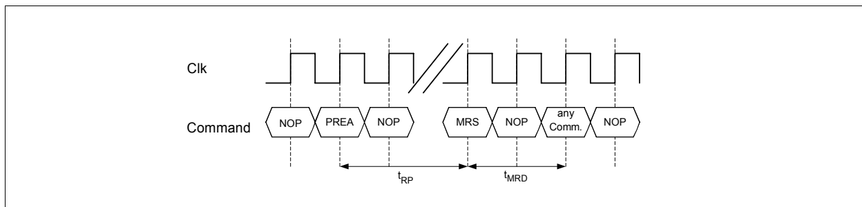
Figure 10 Mode Register Set Timing
