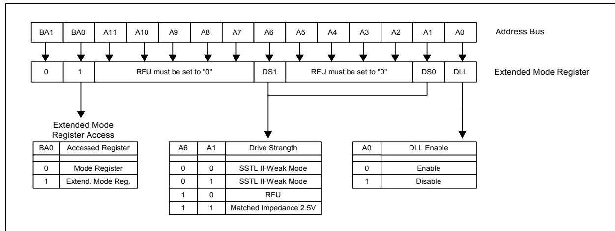
Figure 4 Extended Mode Register Bitmap
