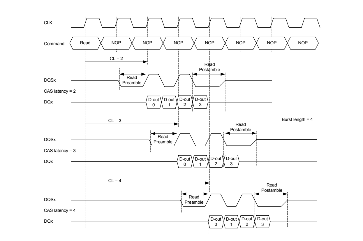
Figure 17 Burst Read Operation
