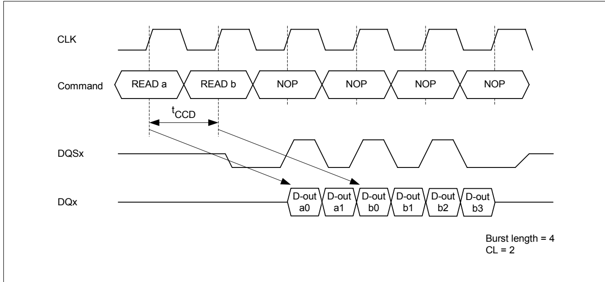
Figure 24 Read interrupted by Read
