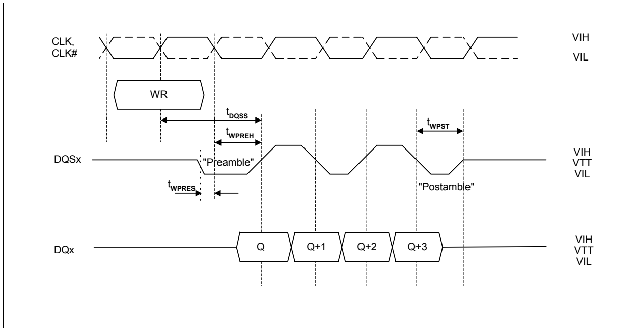
Figure 8 DQS Pre/Postamble at Write
