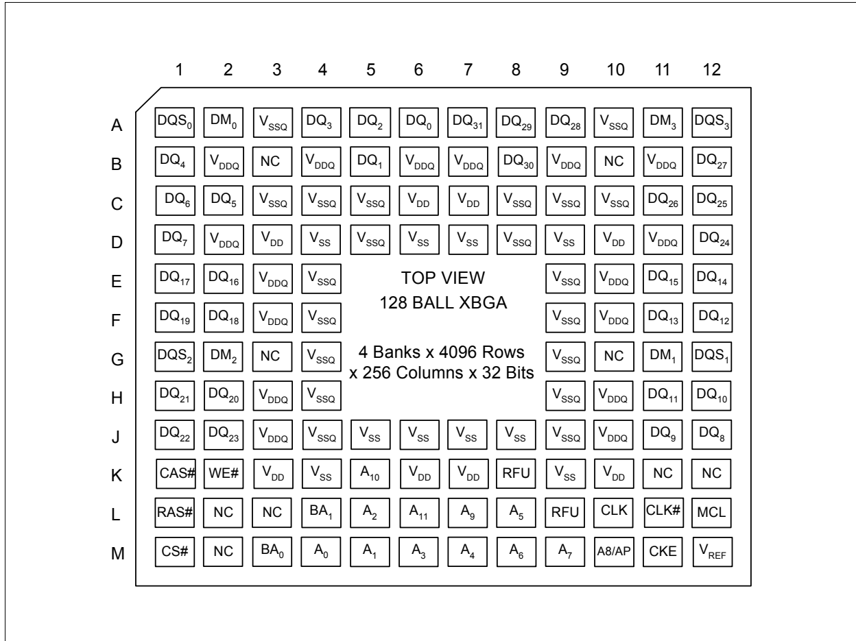
Figure 1 Ball Out 128Mbit DDR SGRAM
