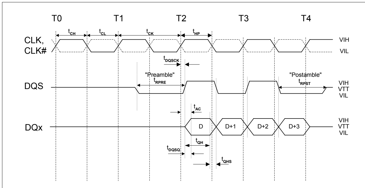
Figure 6 DQS Timing for Read
