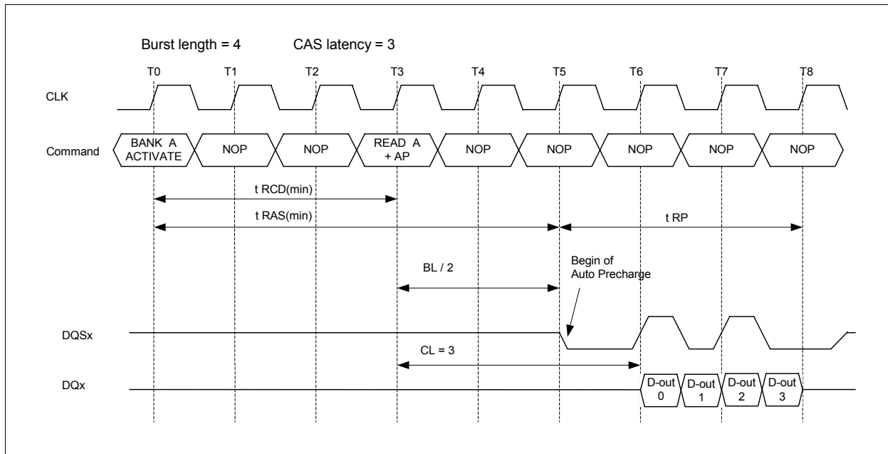
Figure 22 Read Concurrent Auto Precharge
