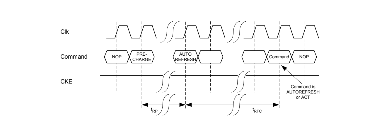
Figure 15 Autorefresh timing
