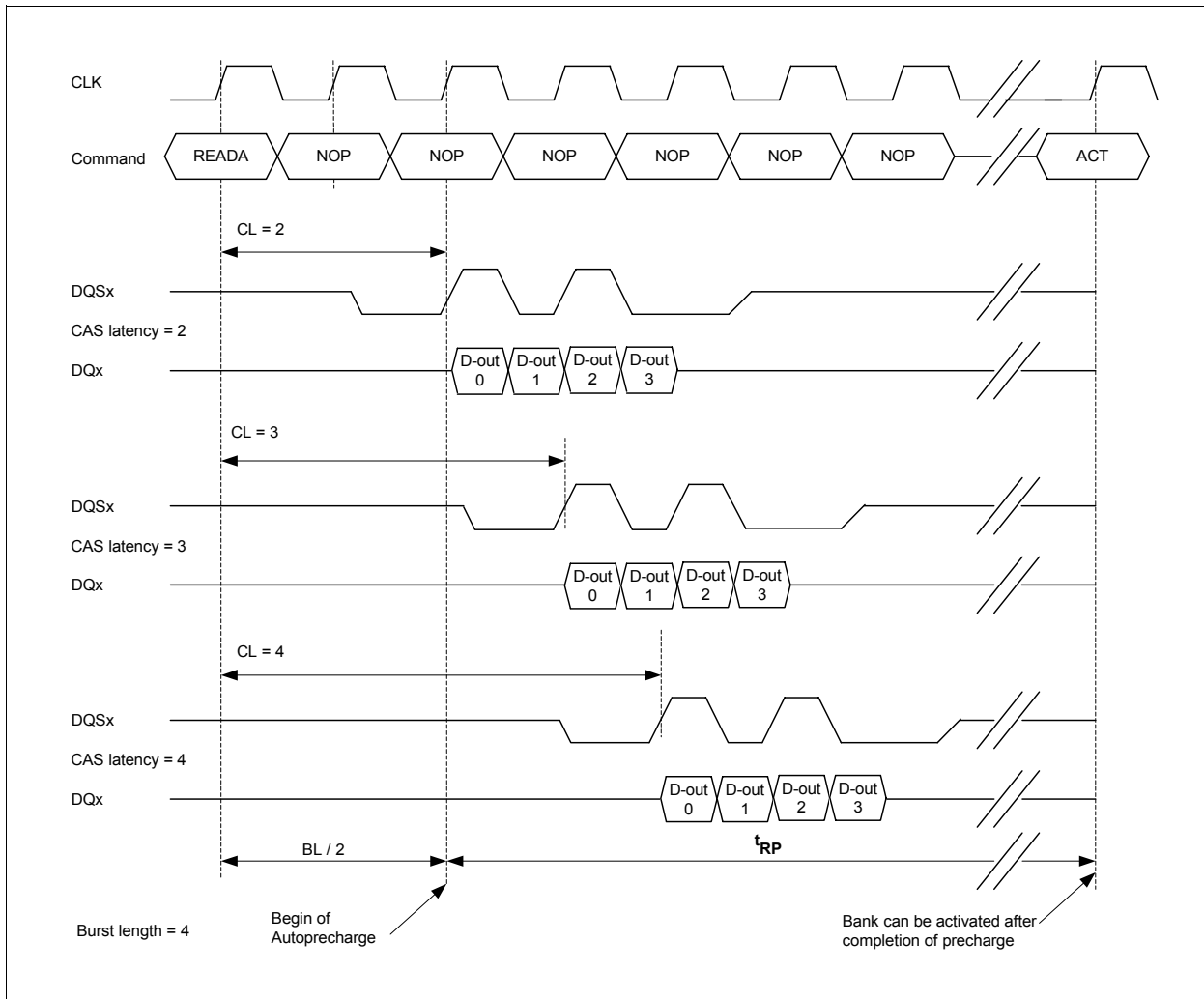
Figure 21 Read Burst with Autoprecharge
