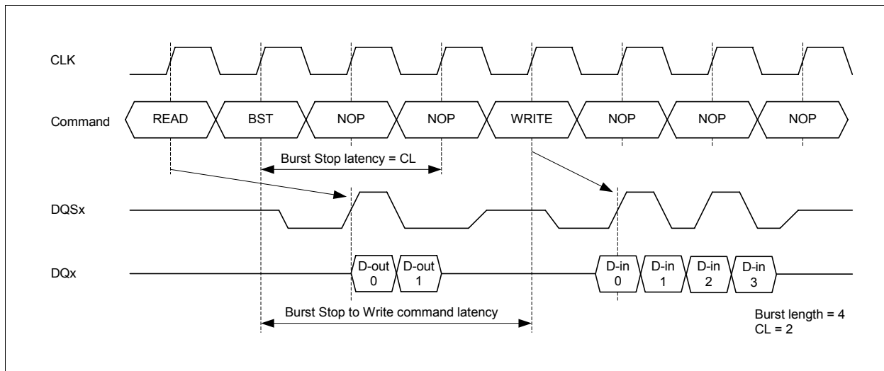
Figure 25 Read interrupted by Write
