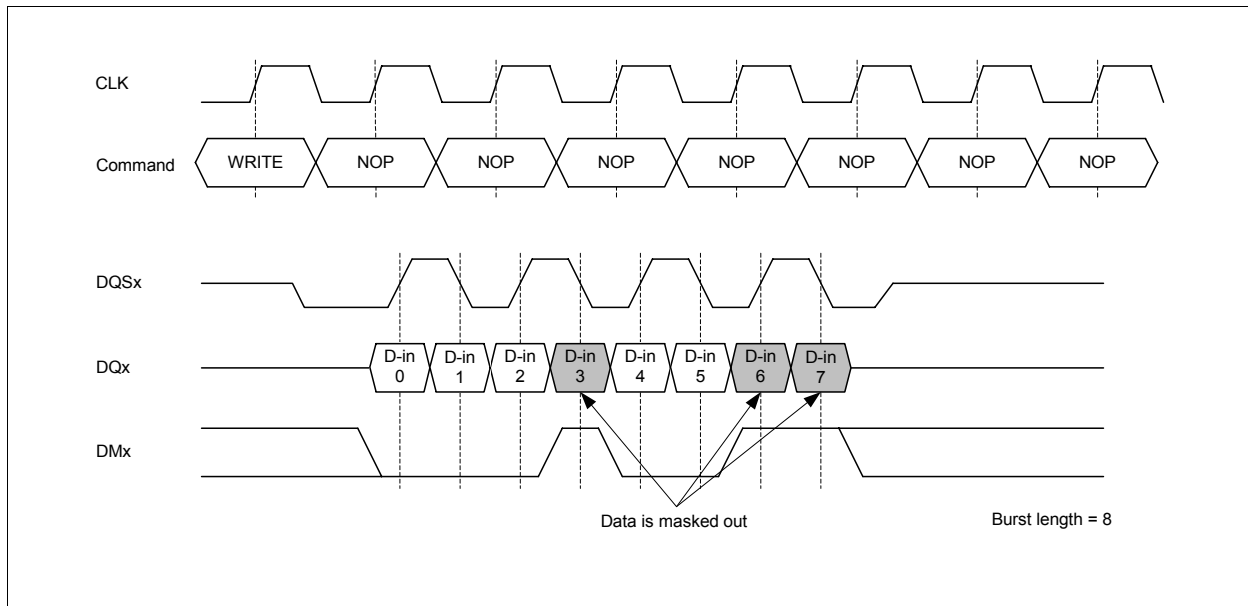
Figure 20 Data Mask Timing
