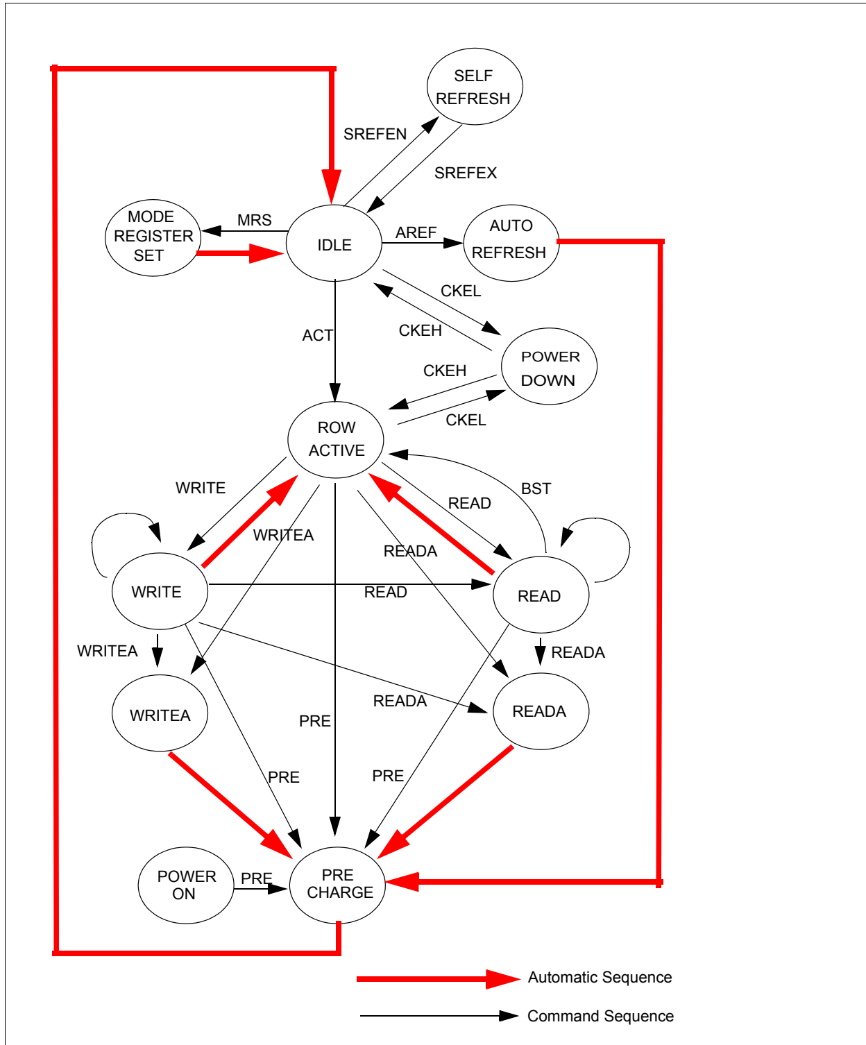
Figure 30 DDR SGRAM Simplified State Diagram
