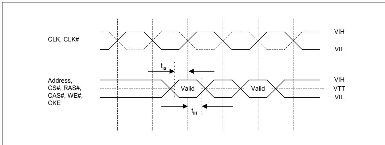
Figure 5 Command and Address Signal Timing
