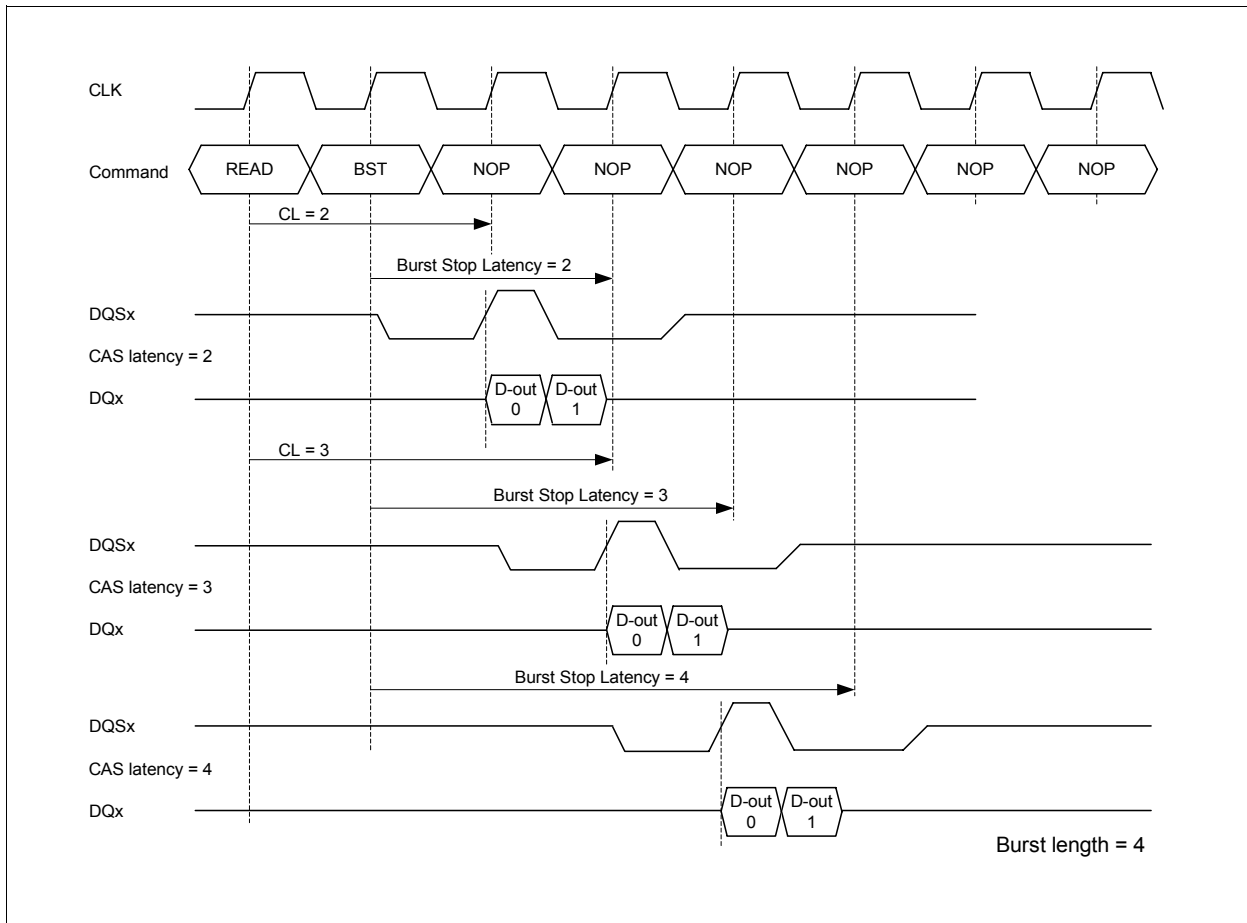
Figure 19 Burst Stop for Read
