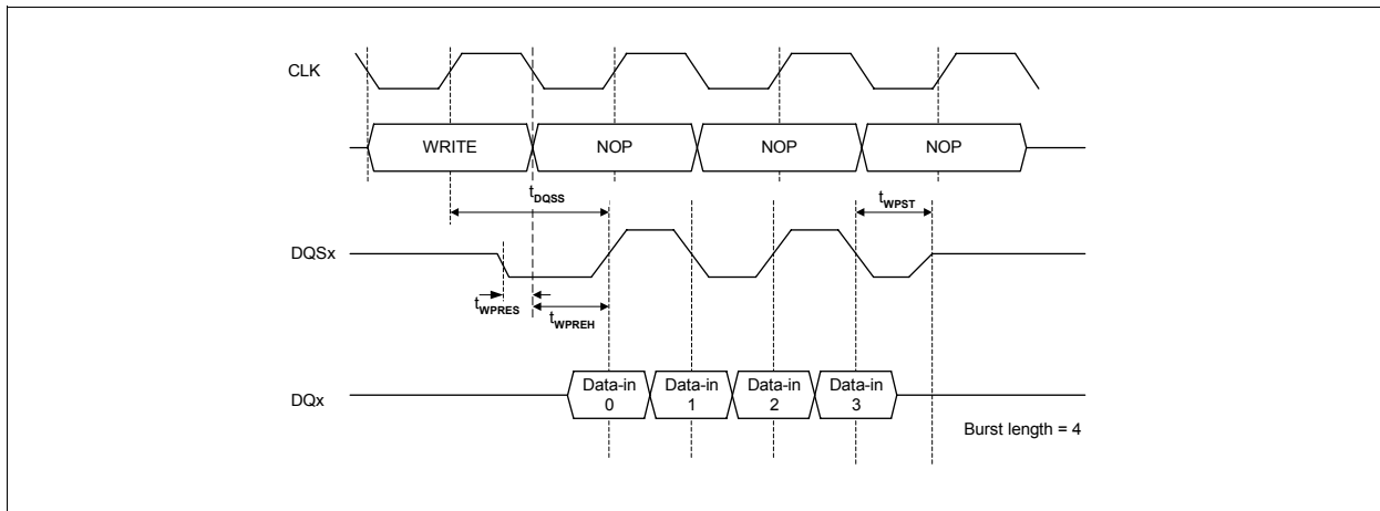
Figure 18 Burst Write Operation
