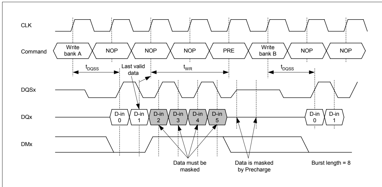
Figure 29 Write interrupted by Precharge
