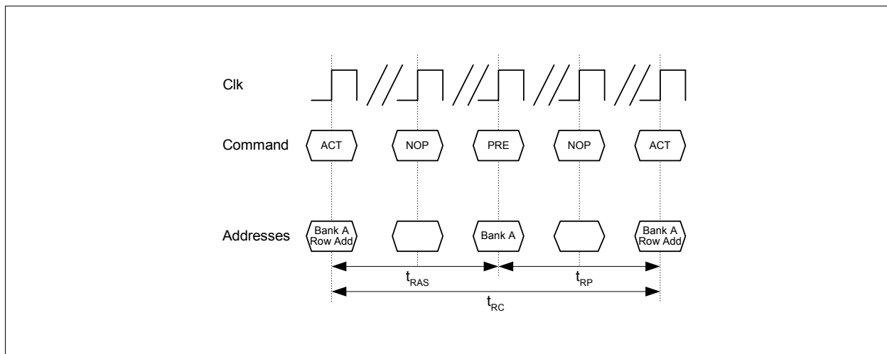
Figure 13 Precharge Command Timing
