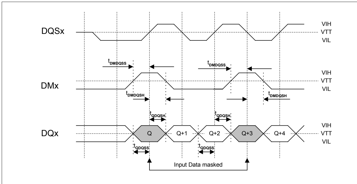
Figure 7 DQS and DM Timing at Write
