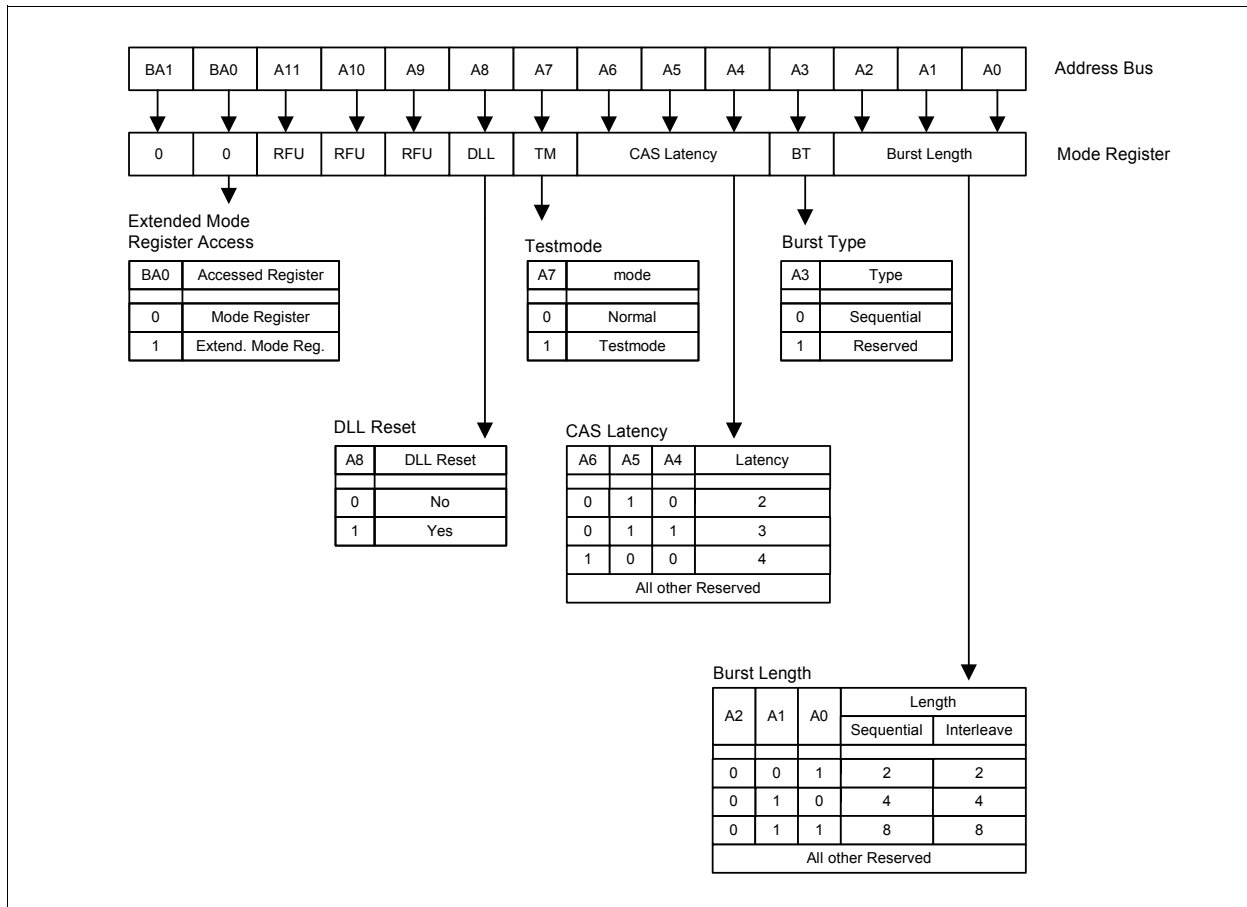
Figure 3 Mode Register Bitmap
