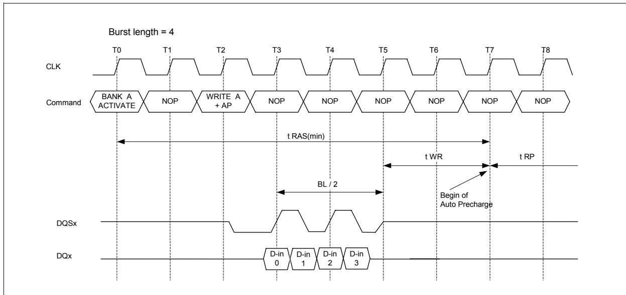
Figure 23 Write Burst with Auto Precharge
