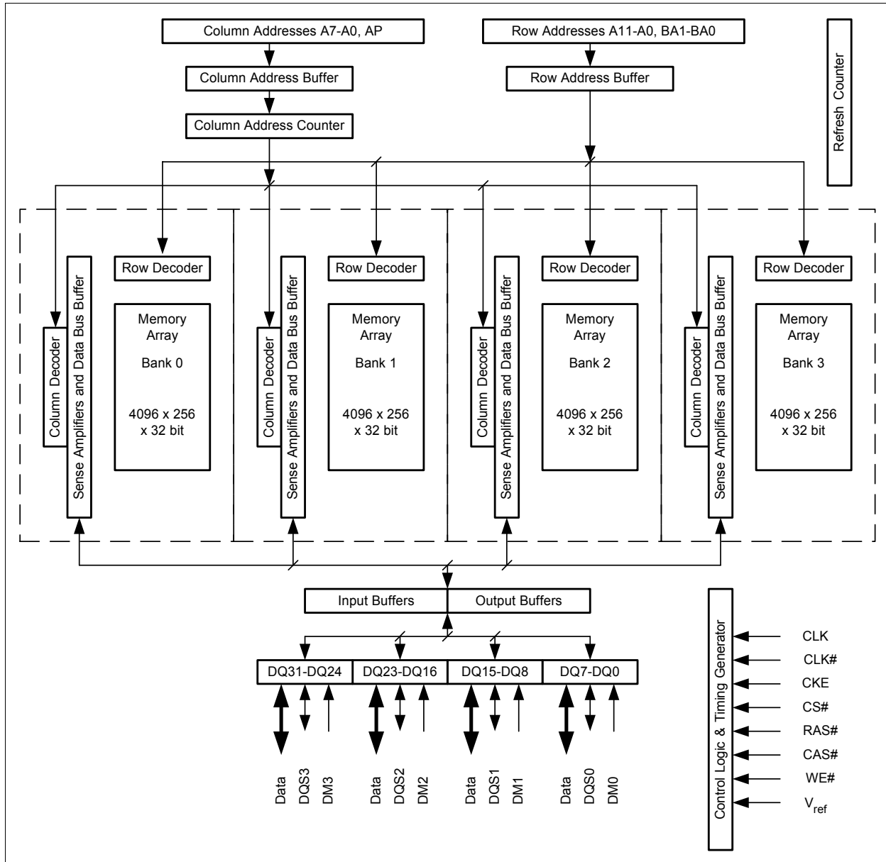
Figure 2 Functional blocks
