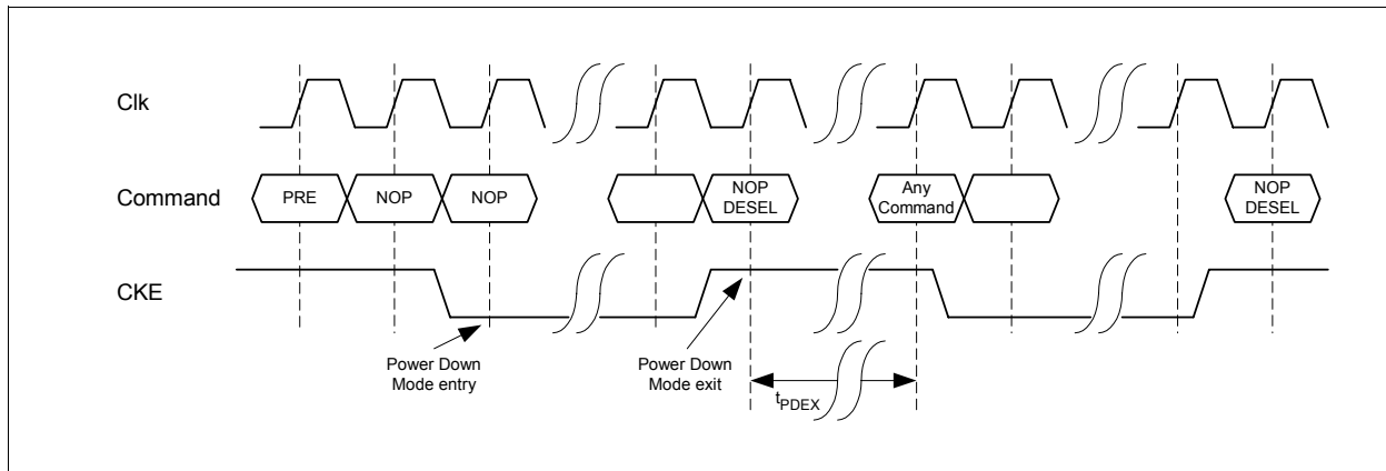
Figure 16 Power Down Mode timing
