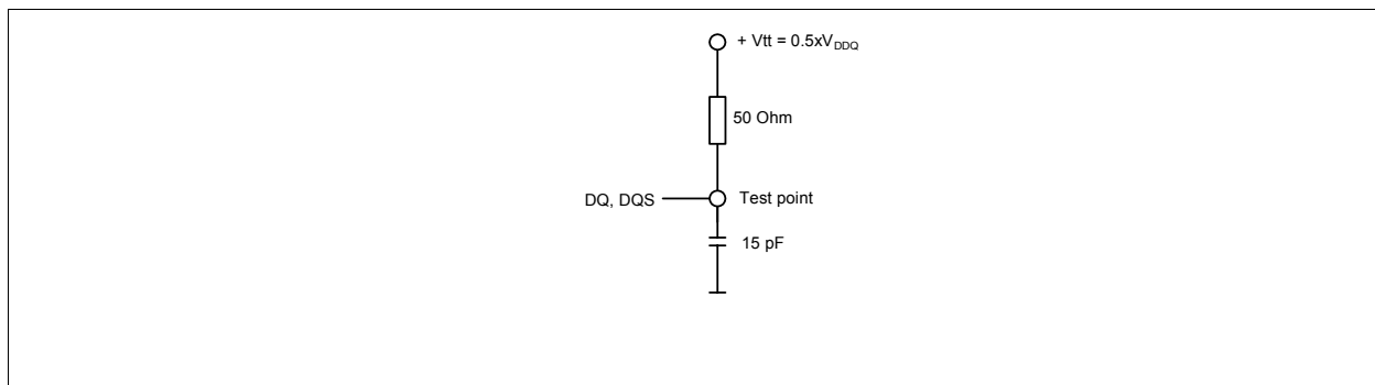
Figure 31 Output Test Circuit
