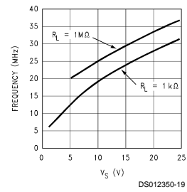
Unity Gain Frequency vs. Supply Voltage for Various Loads
