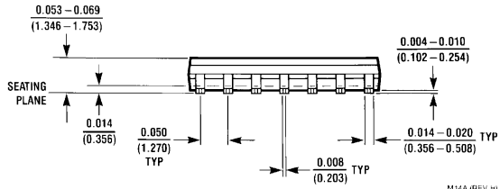
14-Lead Small Outline Molded Package (M) Order Number DM74LS30M NS Package Number M14A
