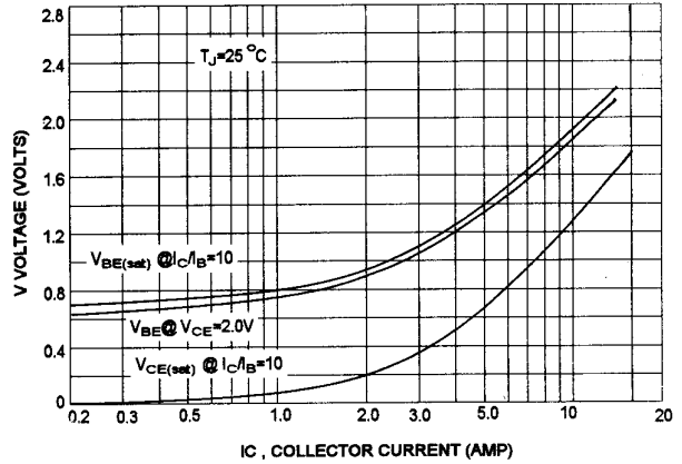
"ON" VOLTAGES
