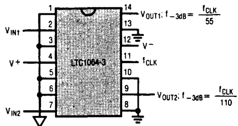
Figure 6. Dual 4th Order Bessel Filters. V_S = \pm 7.5V , f_{CLK} = 1MHz , Pin 10 to GND. f_{-3dB} = 9kHz and 18kHz .
