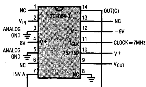
8th Order Clock Sweeable Lowpass Bessel Filter
