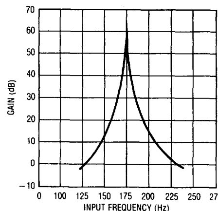
Amplitude Response
