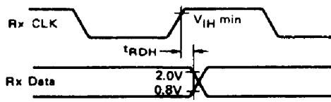
Figure 5 Receive Data Hold Time (÷1 Mode)
