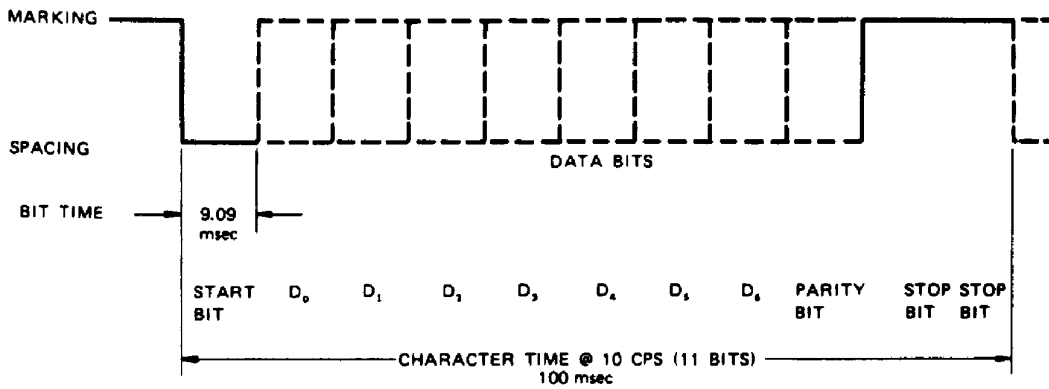
Figure 10 110 Baud Serial ASCII Data Timing
