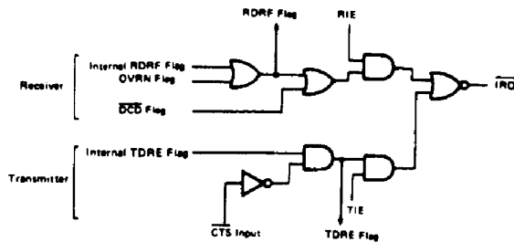
Figure 14 \overline{\text{IRQ}} Internal Circuit
