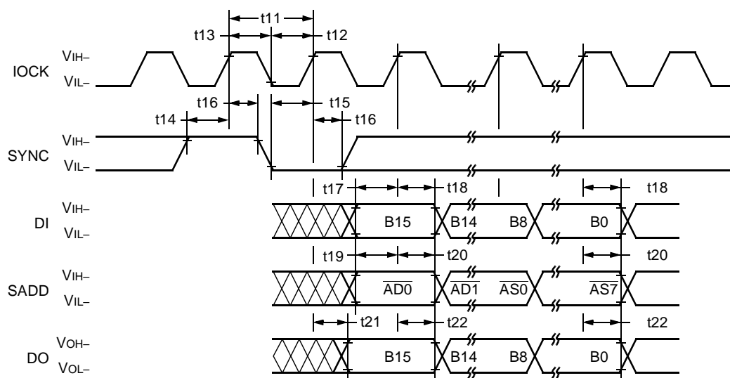
Figure 42. Serial Input/Output Timing Diagram
