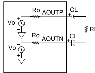
B. Fully Differential, with Capacitive Coupling
