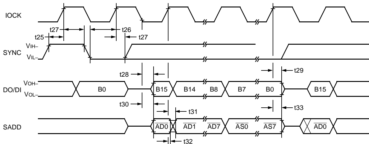
Figure 44. SIO Multiprocessor Timing Diagram
