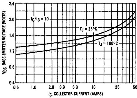
FIGURE 13 — BASE-EMITTER SATURATION VOLTAGE
