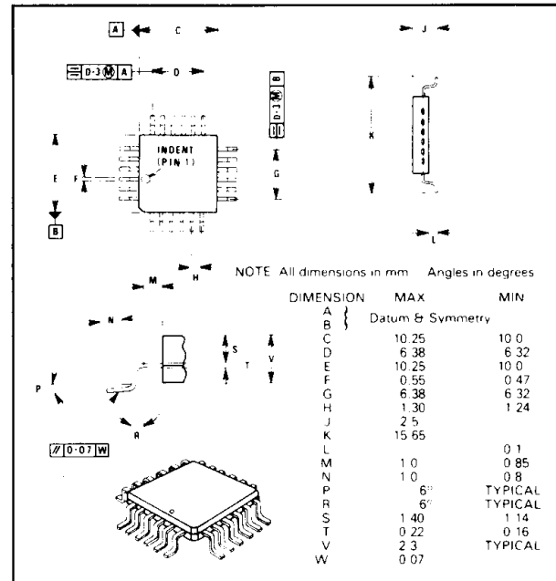
Fig. 8 FX316LH Package
