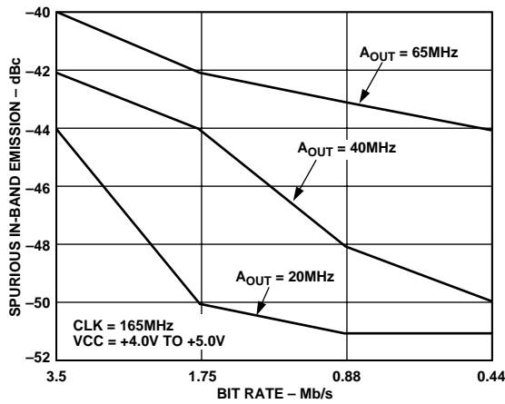
Figure 25. Spurious Emission vs. Bit Rate vs. A OUT
