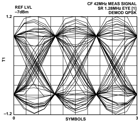
Figure 16. QPSK Modulation
