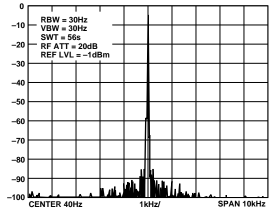
Figure 14. 6x REFCLK Disabled
