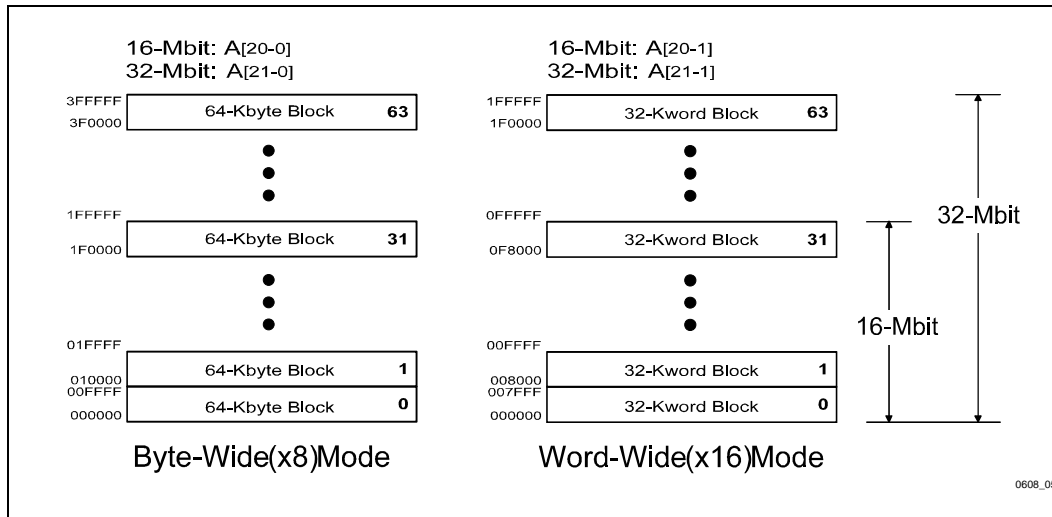
Figure 4. Memory Map
