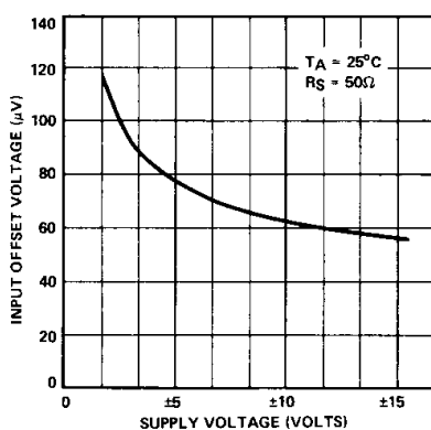
INPUT OFFSET VOLTAGE vs POWER SUPPLY VOLTAGE
