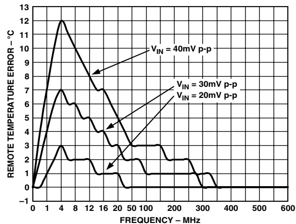
TPC 7. Remote Temperature Error vs. Differential-Mode Noise Frequency
