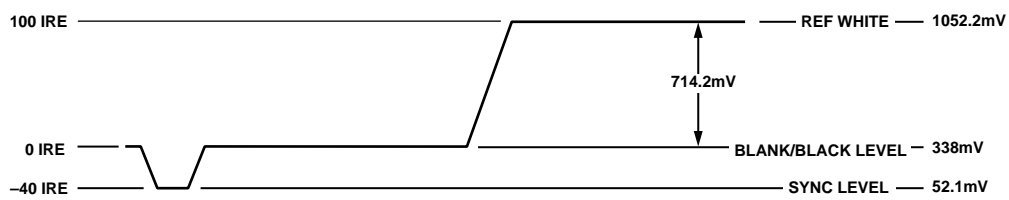
Figure 66. NTSC Luma Video Levels
