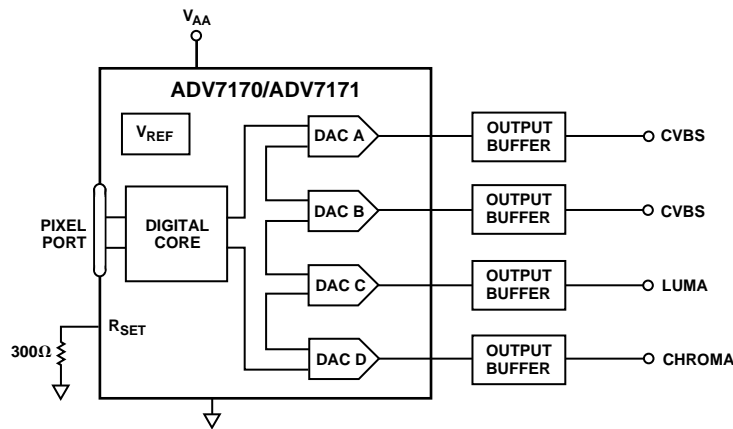
Figure 83. Output DAC Buffering Configuration
