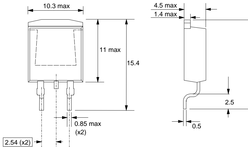
Fig.20. SOT404 : centre pin connected to mounting base.
