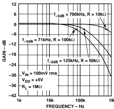
Figure 23. -3 dB Bandwidths
