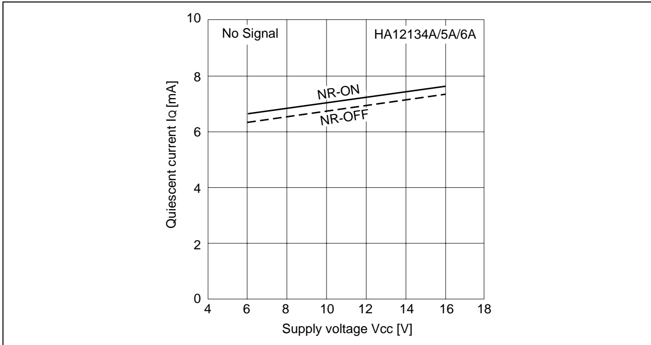
Figure 1 Quiescent Current vs. Supply Voltage
