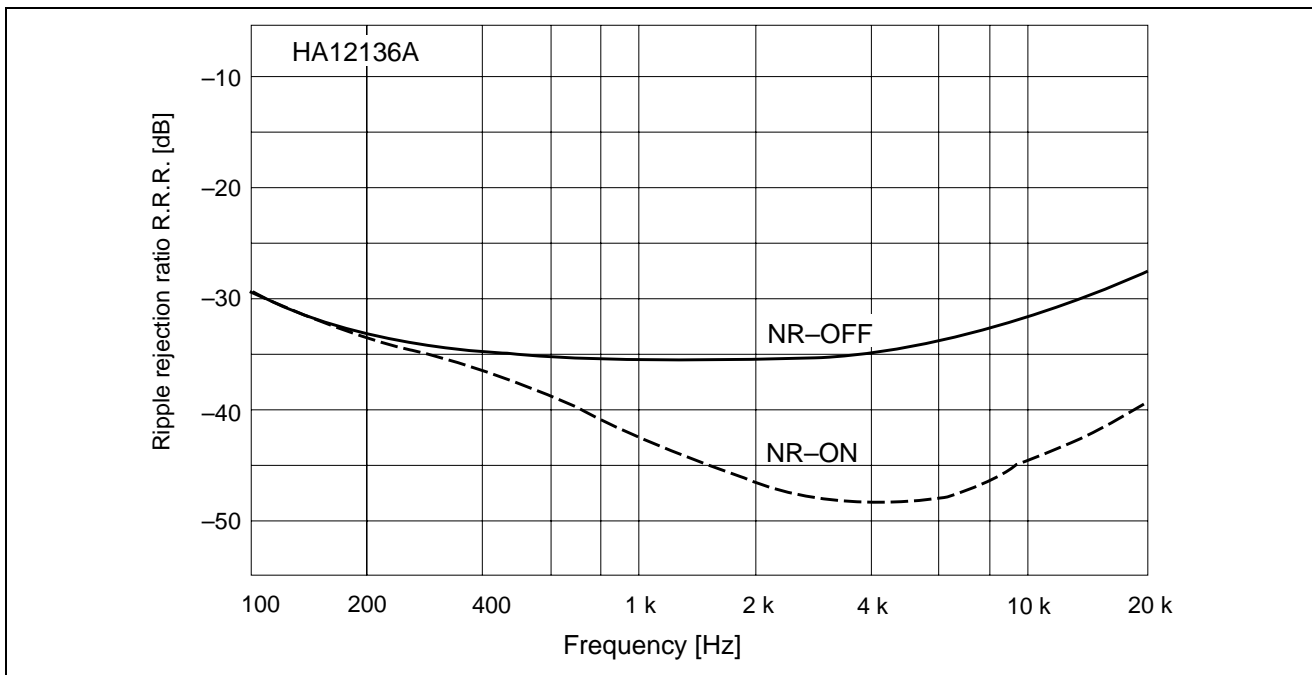
Figure 8 PB Mode Ripple Rejection Ratio vs. Frequency
