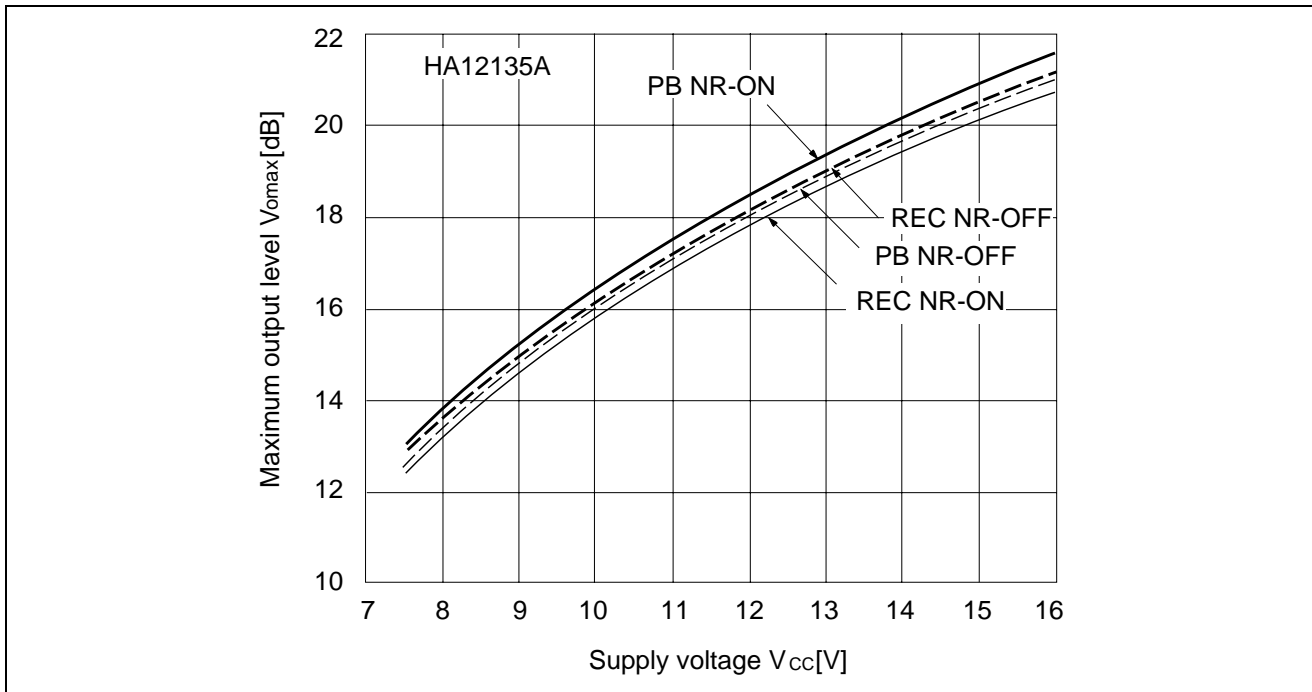
Figure 24 Maximum Output Level vs. Supply Voltage
