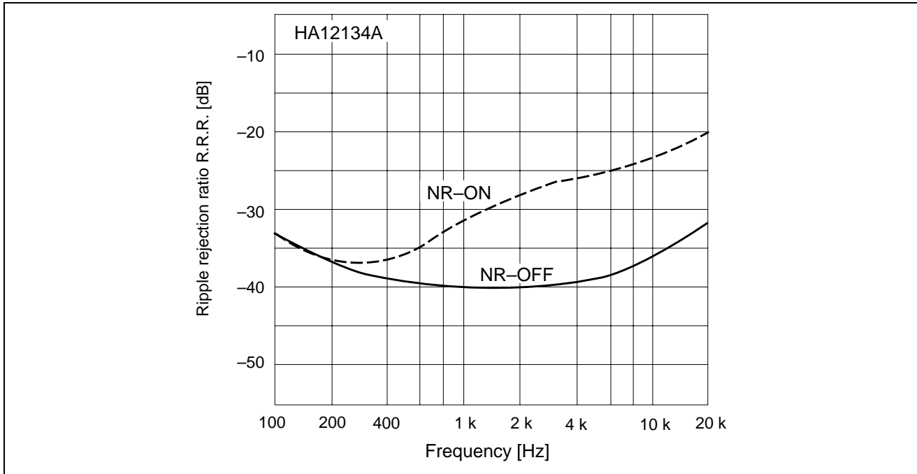
Figure 29 REC Mode Ripple Rejection Ratio vs. Frequency
