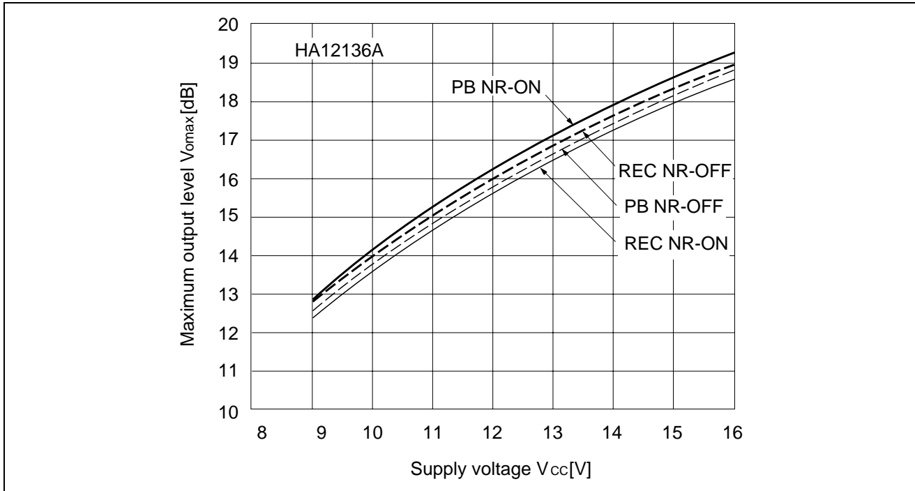
Figure 13 Maximum Output Level vs. Supply Voltage
