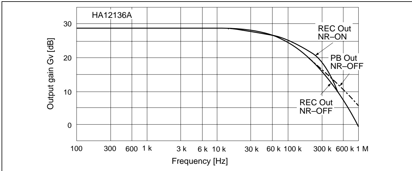
Figure 6 PB Mode Output Gain vs. Frequency
