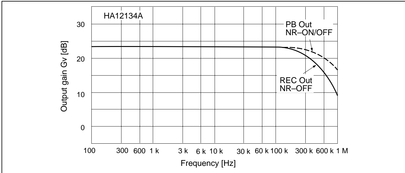
Figure 27 REC Mode Output Gain vs. Frequency
