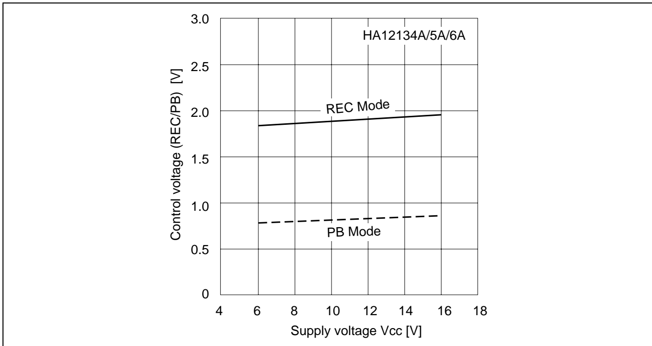
Figure 2 REC/PB Control Voltage vs. Supply Voltage
