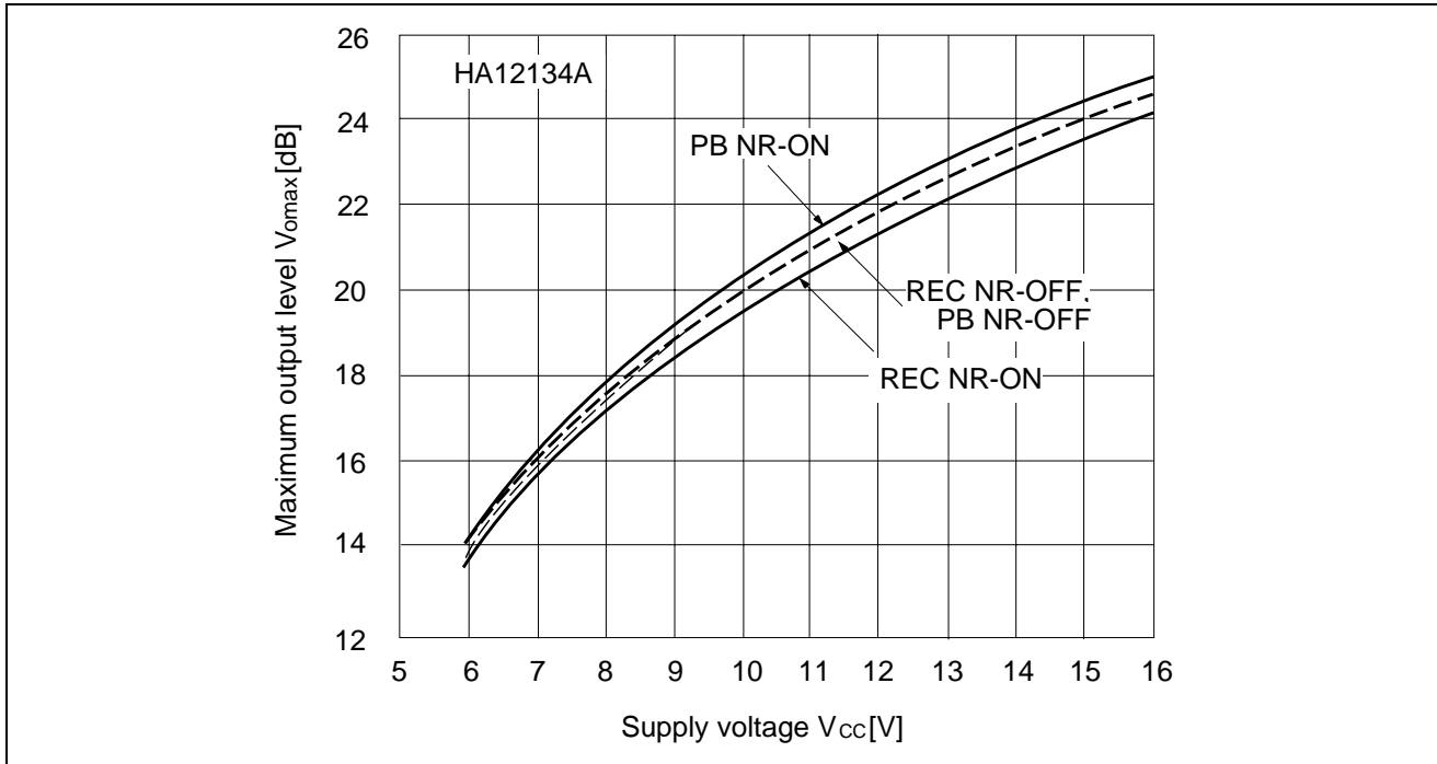
Figure 35 Maximum Output Level vs. Supply Voltage
