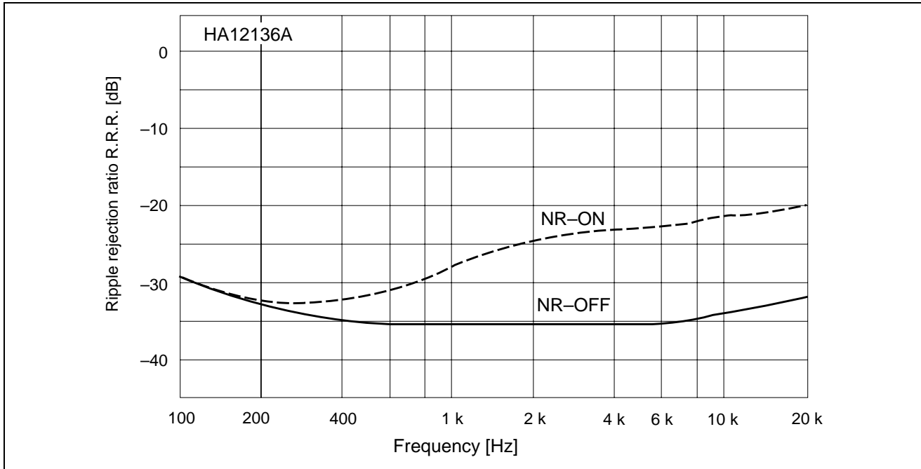
Figure 7 REC Mode Ripple Rejection Ratio vs. Frequency
