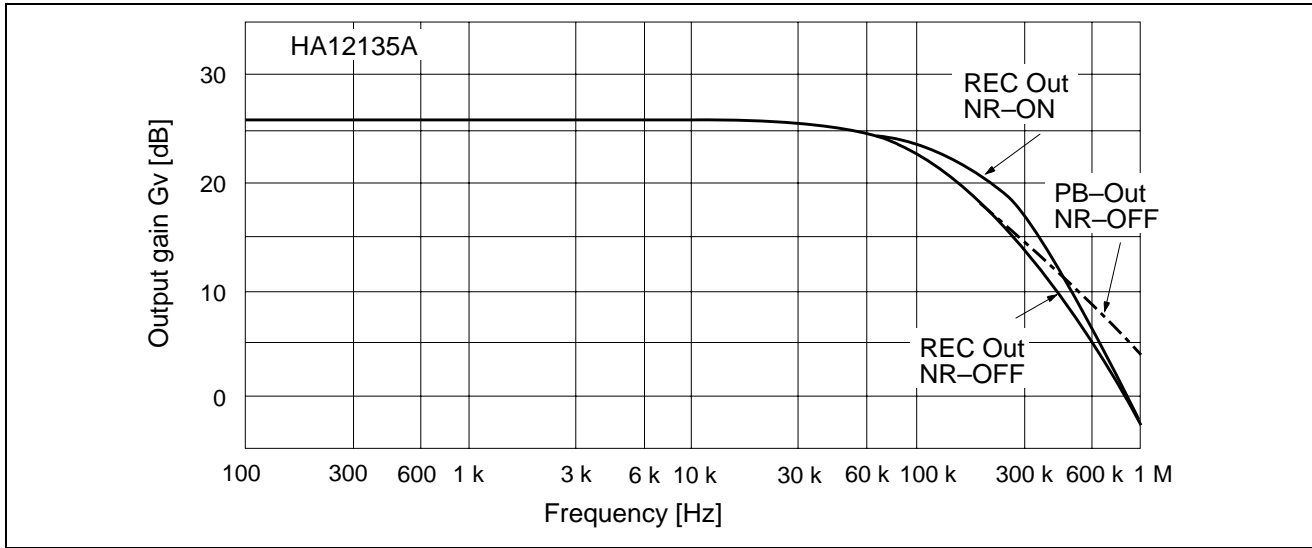
Figure 17 PB Mode Output Gain vs. Frequency
