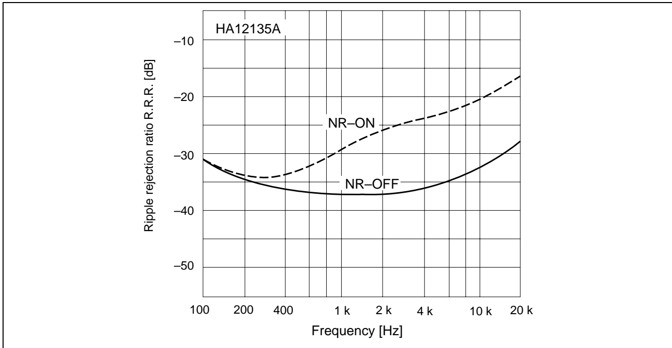
Figure 18 REC Mode Ripple Rejection Ratio vs. Frequency
