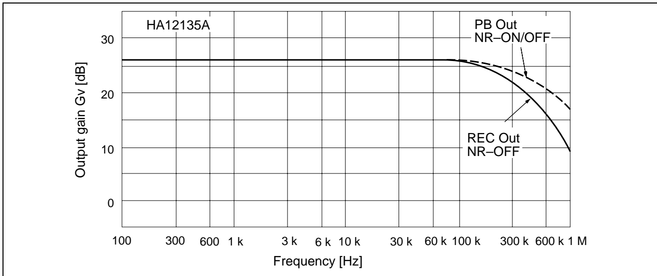
Figure 16 REC Mode Output Gain vs. Frequency
