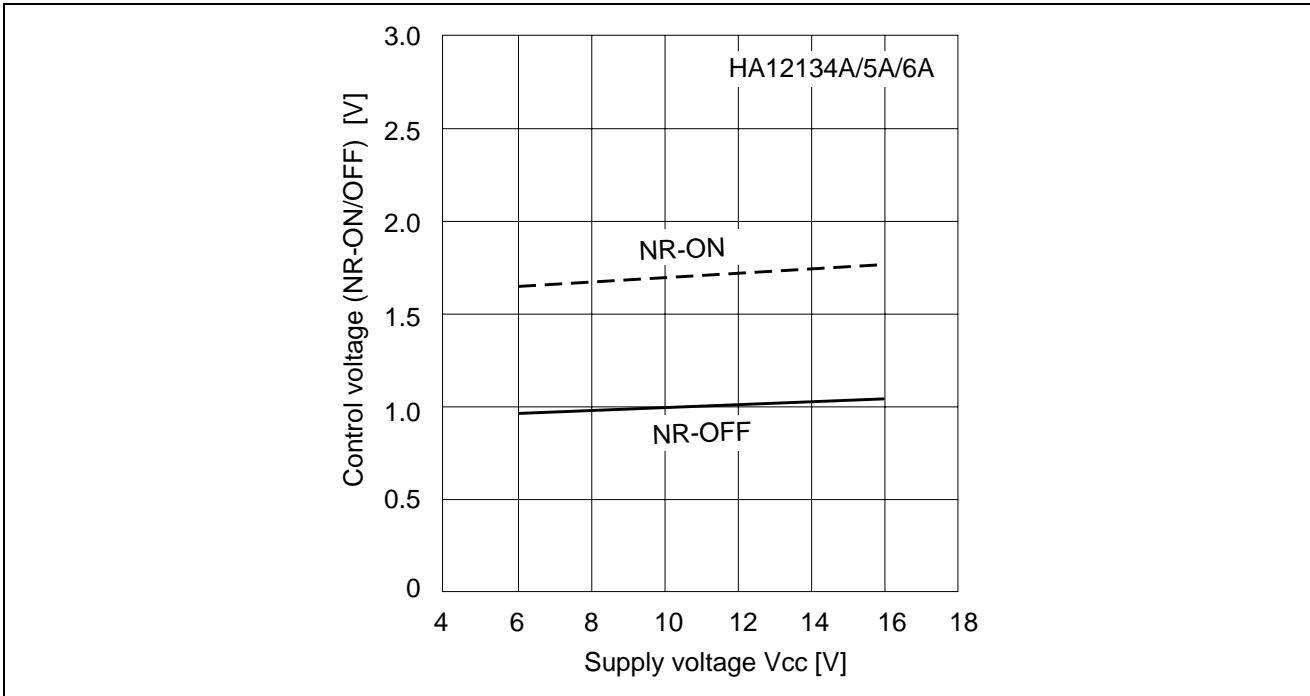
Figure 3 NR-ON/OFF Control Voltage vs. Supply Voltage
