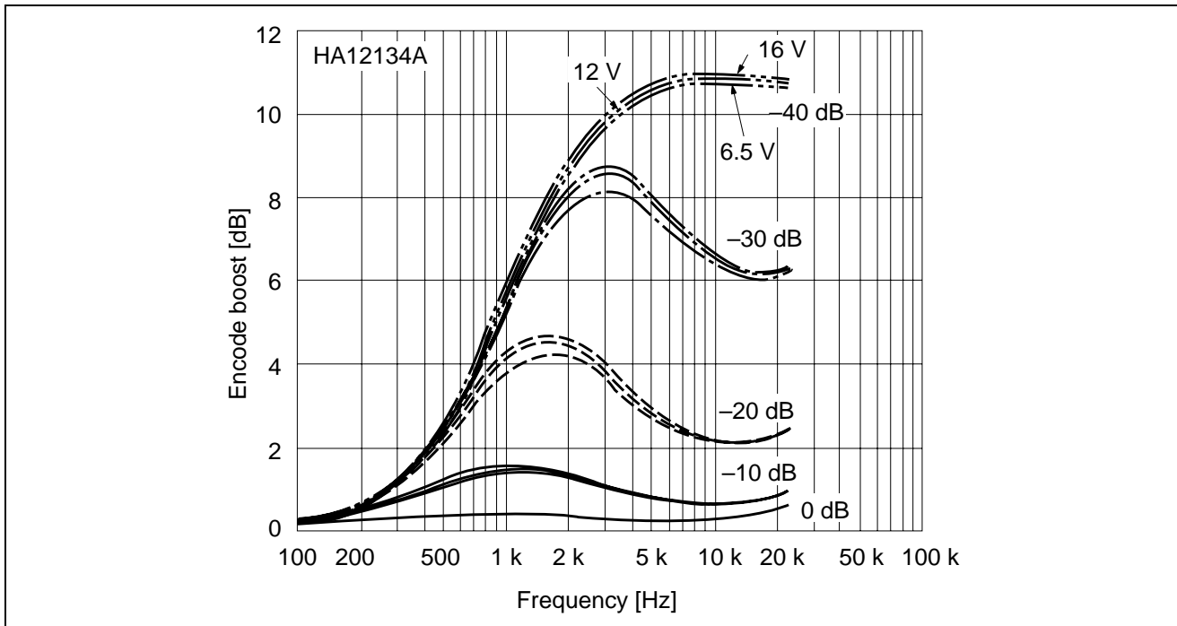
Figure 26 Encode Boost vs. Frequency
