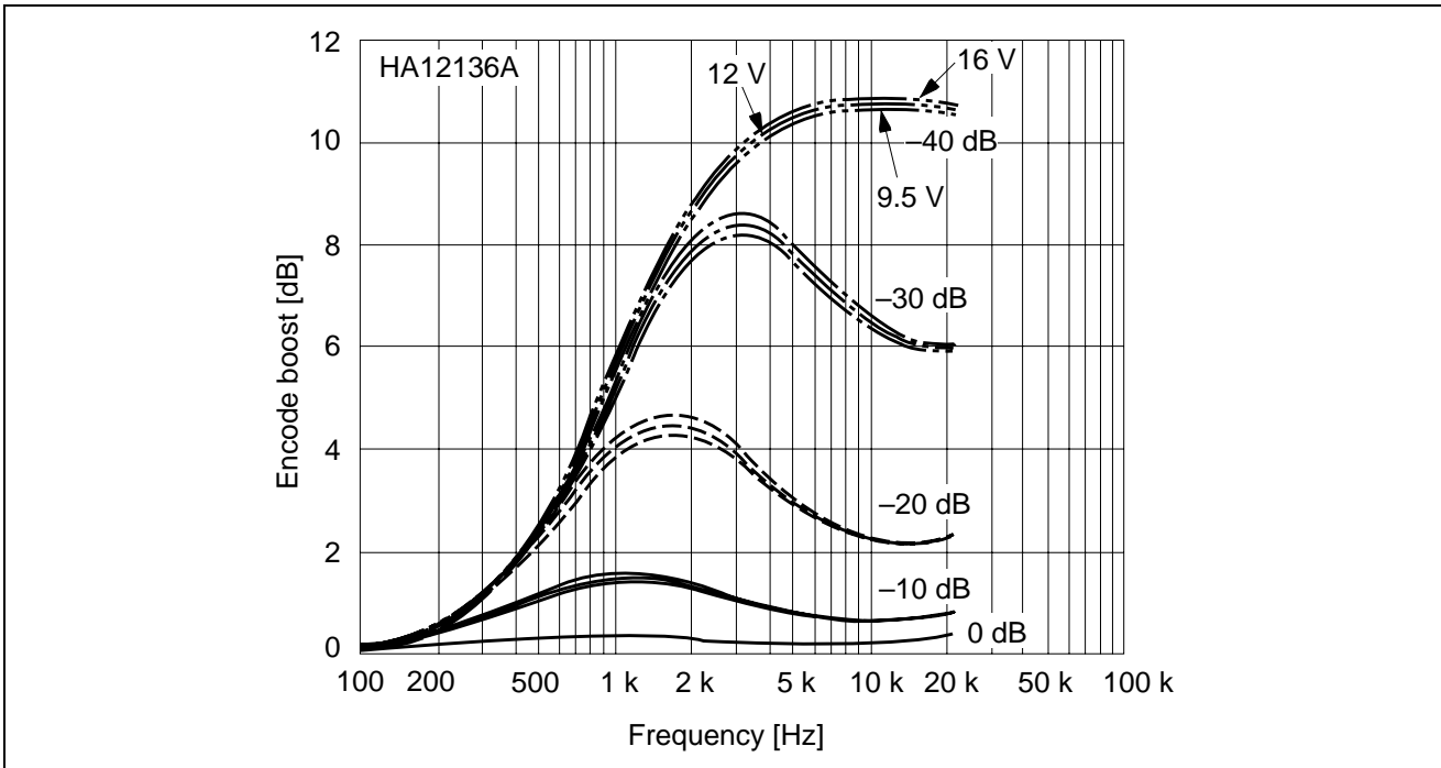
Figure 4 Encode Boost vs. Frequency
