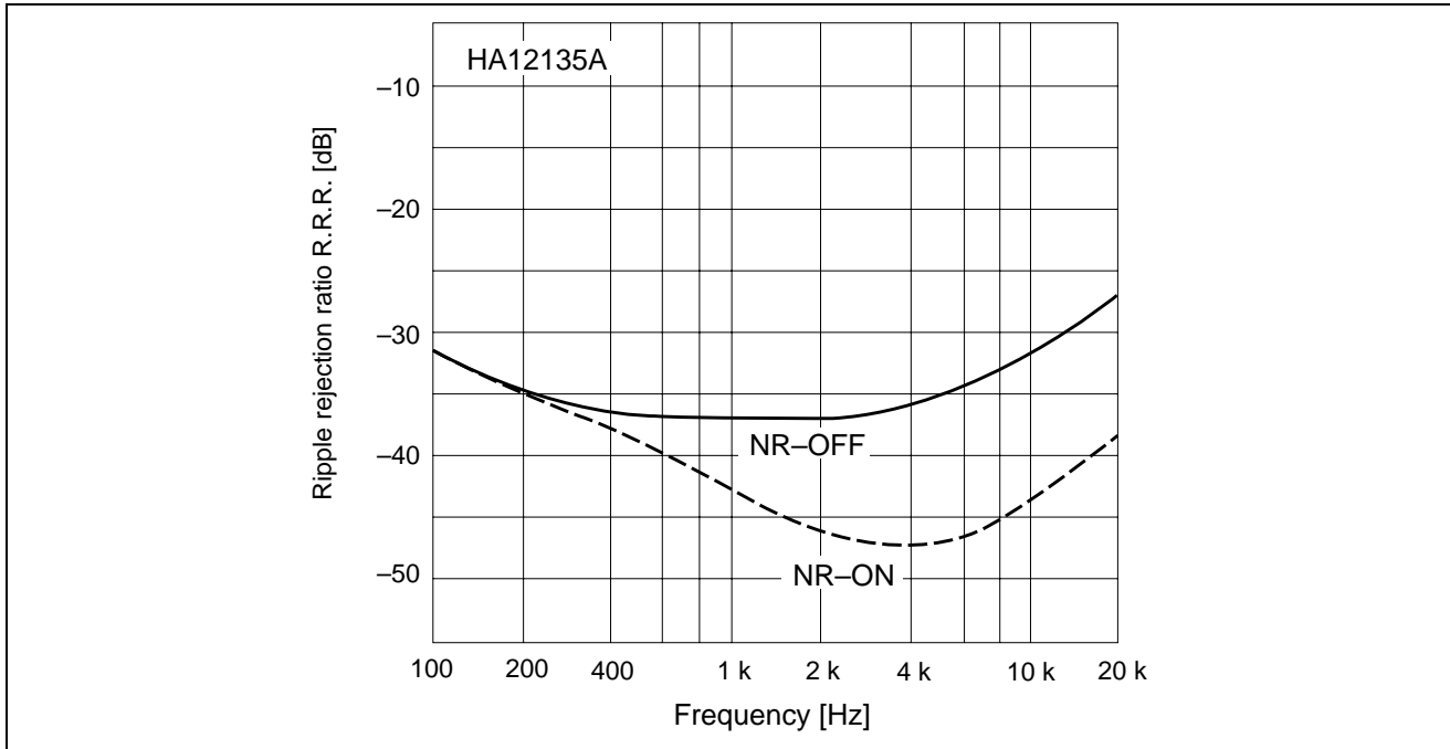
Figure 19 PB Mode Ripple Rejection Ratio vs. Frequency
