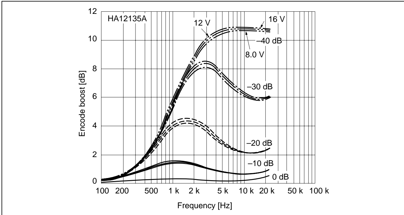
Figure 15 Encode Boost vs. Frequency
