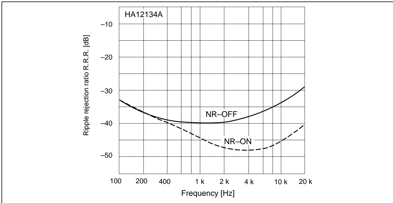
Figure 30 PB Mode Ripple Rejection Ratio vs. Frequency
