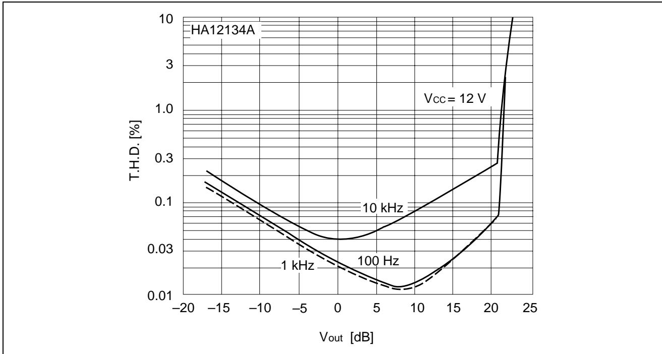
Figure 31 REC NR-OFF Total Harmonic Distortion vs. Output Level
