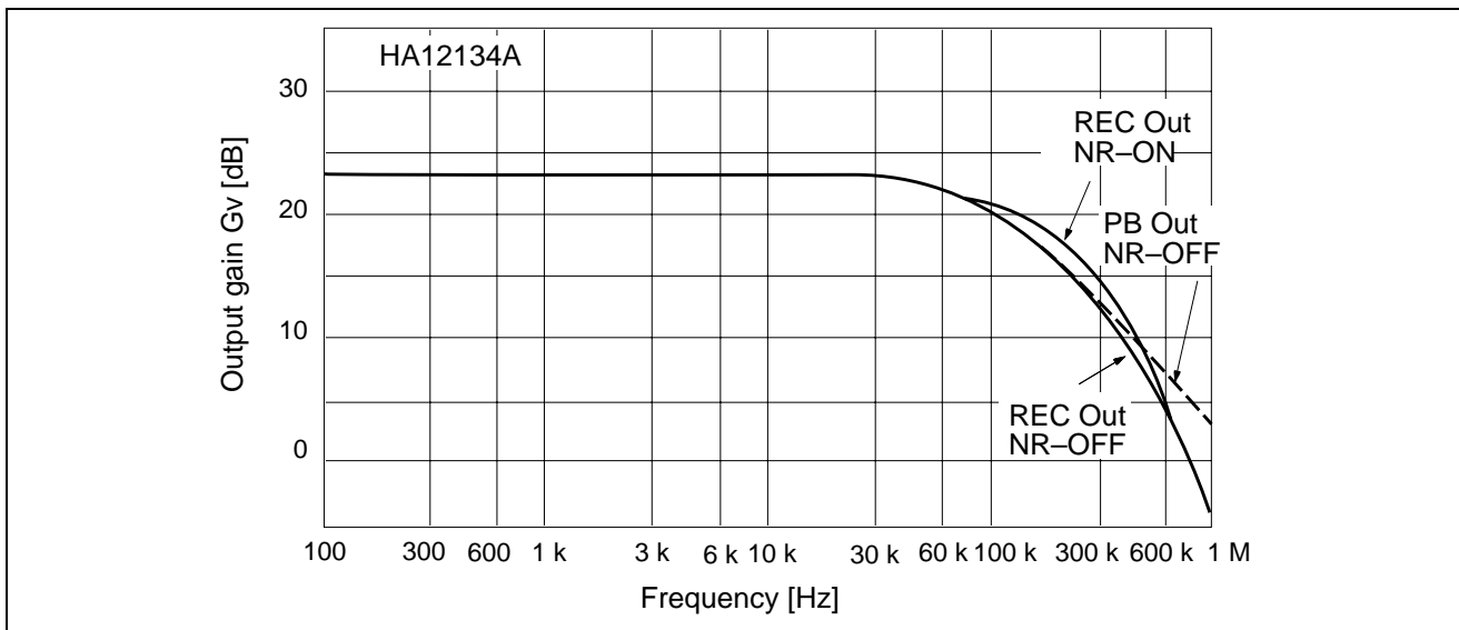
Figure 28 PB Mode Output Gain vs. Frequency
