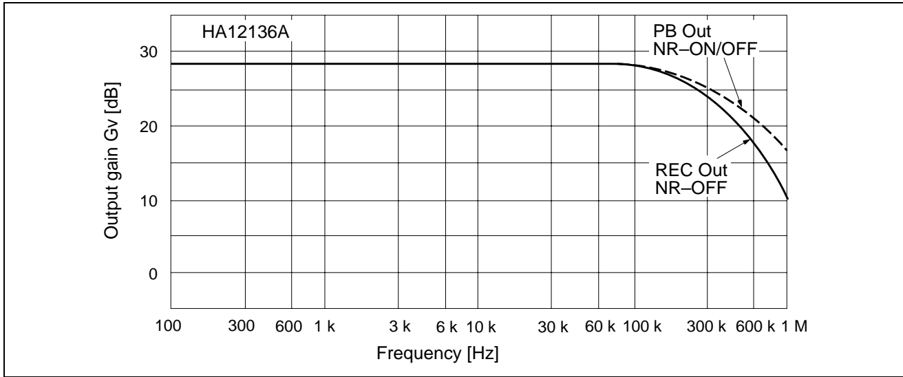
Figure 5 REC Mode Output Gain vs. Frequency
