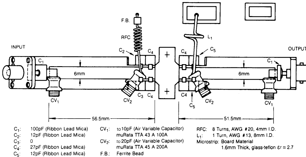
TEST CIRCUIT BOARD LAYOUT (f = 520MHz)
