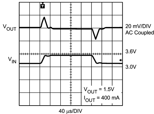
Line Transient Response (PWM Mode)
