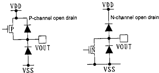
Figure 11 Segment Pin Open Drain Circuit Configurations
