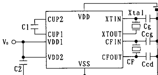
Figure 4 Output Voltage Test Circuit
