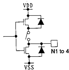
Figure 10 Supply Current Test Circuit
