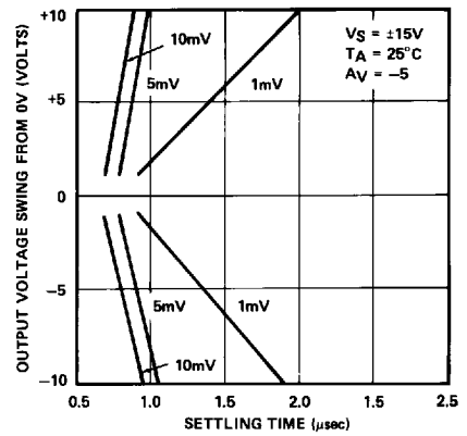
SETTLING TIME
