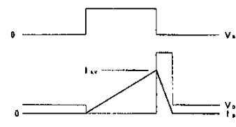
図2 動作波形 Operating waveforms
