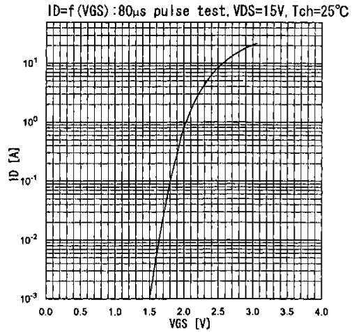
伝達特性 Typical transfer characteristics
