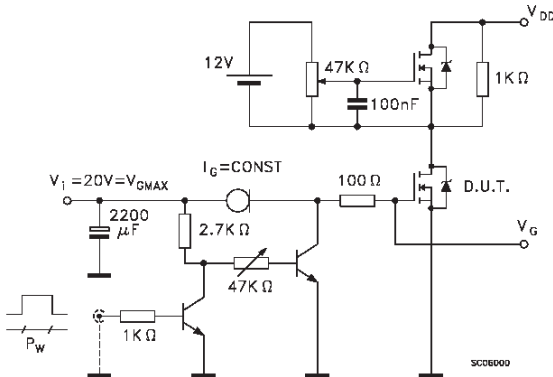
Fig. 2: Gate Charge test Circuit
