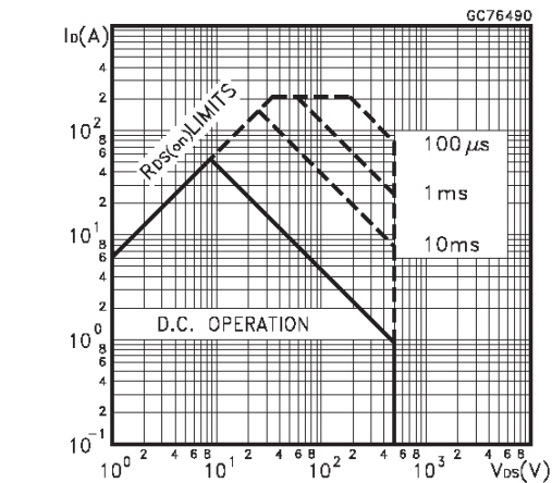
Safe Operating Area for
