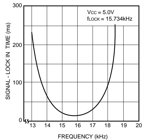
Fig. 19 Time from no signal to pull in
