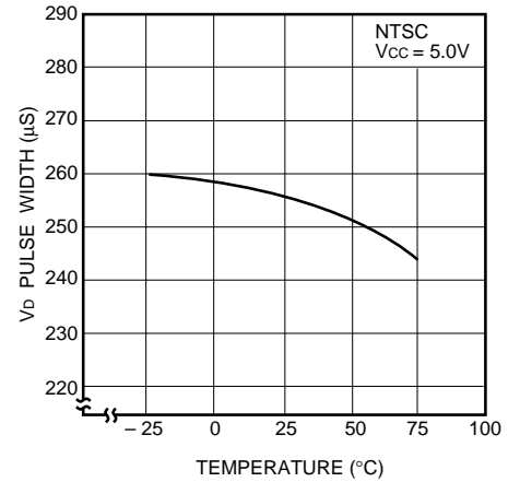
Fig. 16 Vd pulse width vs. temperature
