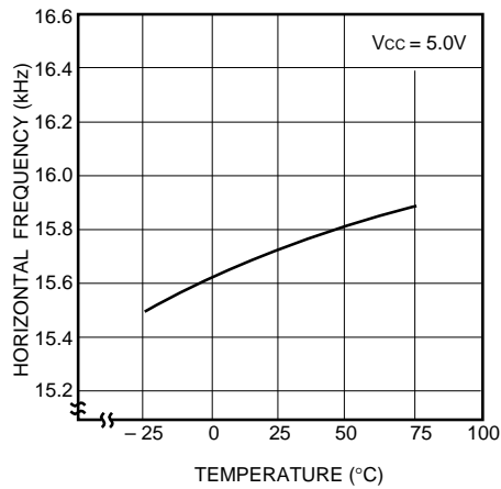
Fig. 14 Horizontal free-running frequency vs. temperature
