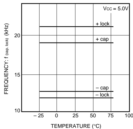
Fig. 18 Capture range / lock range vs. temperature
