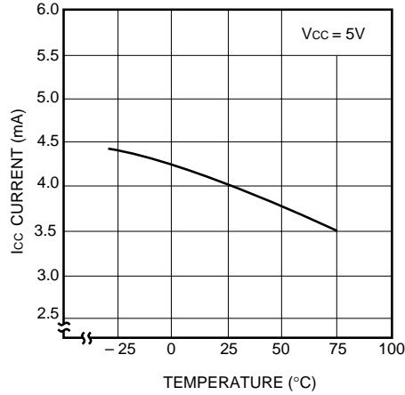
Fig. 12 Quiescent current vs. temperature
