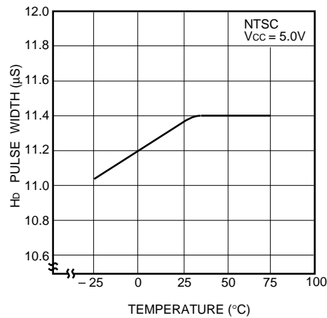
Fig. 15 Hd pulse width vs. temperature
