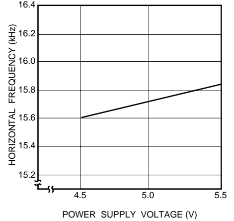
Fig. 13 Horizontal free-running frequency vs. power supply voltage
