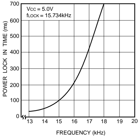
Fig. 20 Time from power on to pull in
