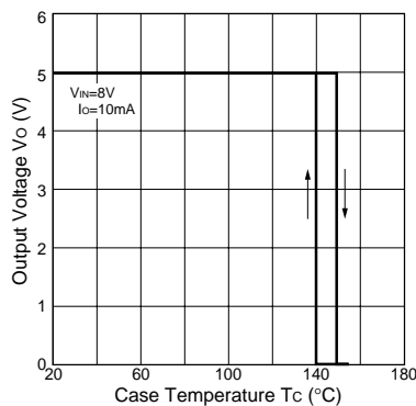
Thermal Protection Characteristics(SI-3051N)
