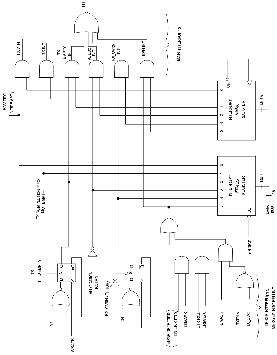
FIGURE 11 - INTERRUPT STRUCTURE
