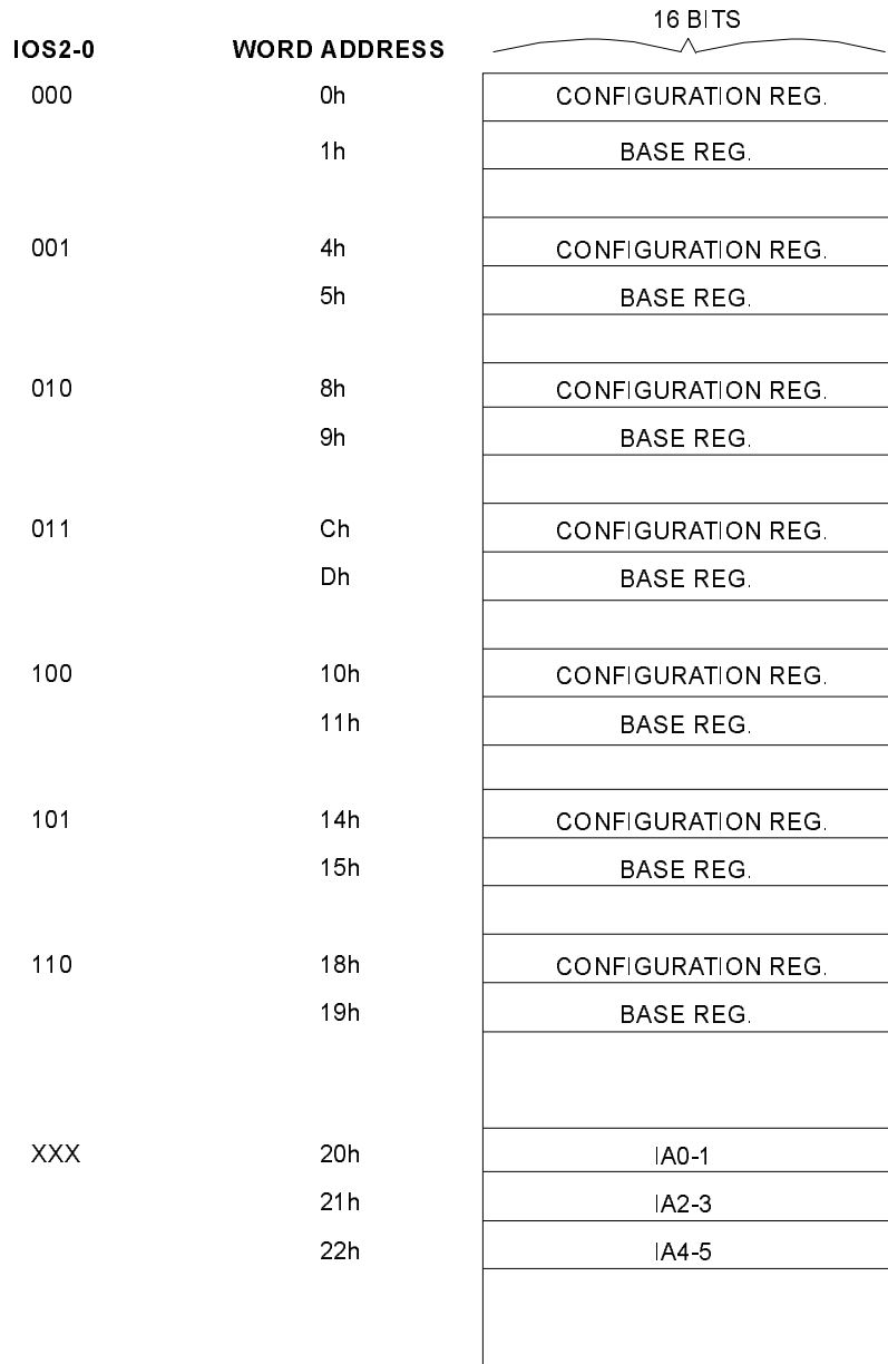
FIGURE 19 - 64 X 16 SERIAL EEPROM MAP
