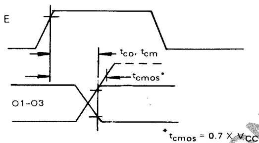
FIGURE 5 — OUTPUT DELAY
