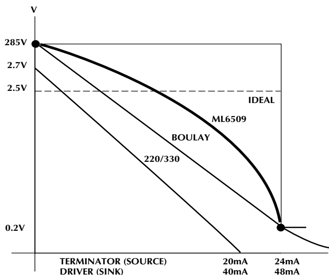
Figure 3. V-1 Characteristics of Various SCSI Termination Schemes
