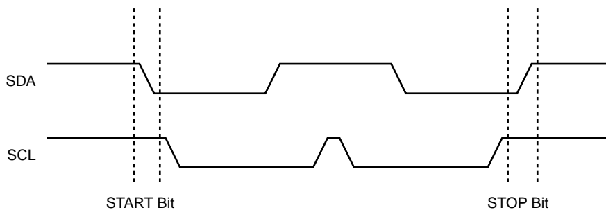
Figure 6. Start/Stop Timing
