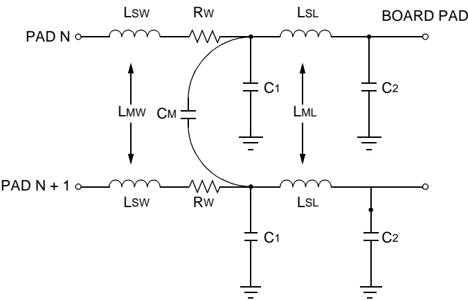
Figure 104. Package Parasitics
