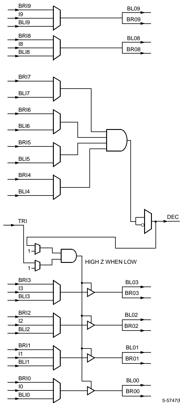
Figure 14. Buffer-Decoder-Buffer Mode
