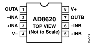
Figure 2. AD8620 8-Lead SOIC
