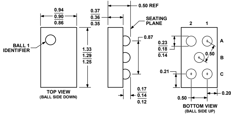
Figure 57. 5-Ball Wafer Level Chip Scale Package [WLCSP] (CB-5) Dimensions shown in millimeters
