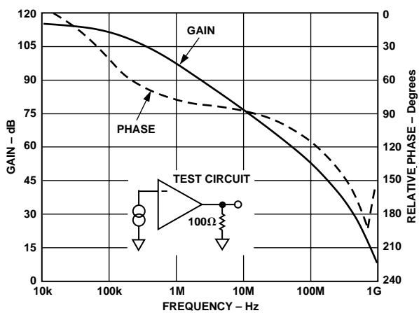
Figure 3. Open Loop Transimpedance Gain [T(s) \text{ Relative to } 1\ \Omega]
