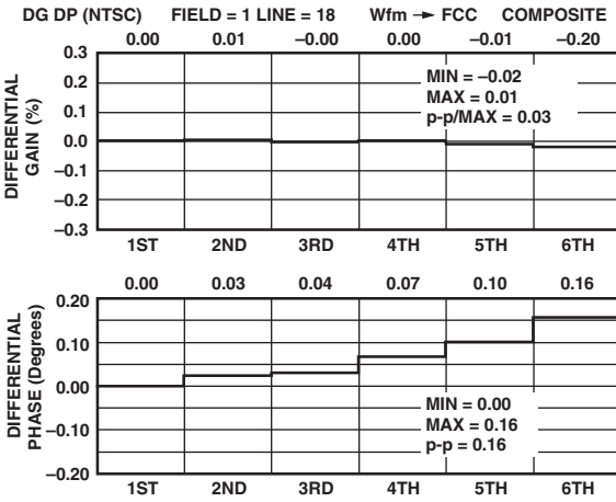
TPC 2. Typical Composite Output Differential Gain and Phase, NTSC for Y Channel; f = 3.58 MHz, R_L = 150 \Omega
