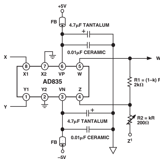
Figure 2. Multiplier Connections
