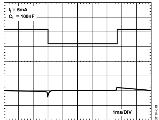
Figure 19. Load Transient
