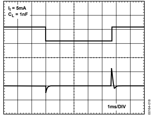
Figure 18. Load Transient
