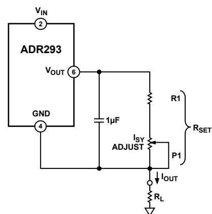
Figure 24. A Precision Current Source
