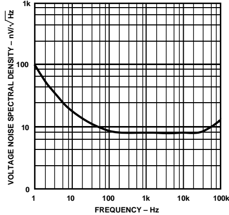
Figure 8. Voltage Noise Spectral Density vs. Frequency
