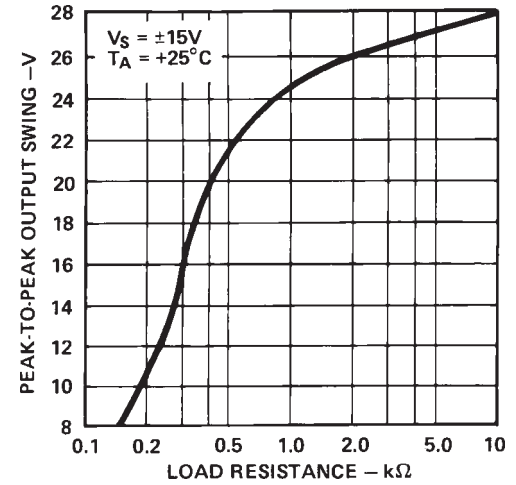
Figure 11. Output Voltage Swing vs. Load Resistance
