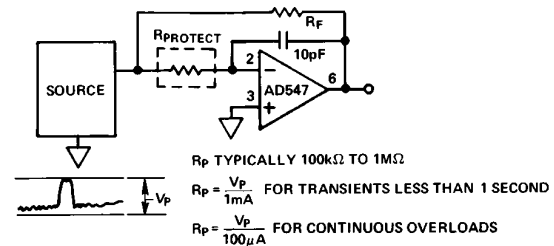
Figure 30. Input Protection
