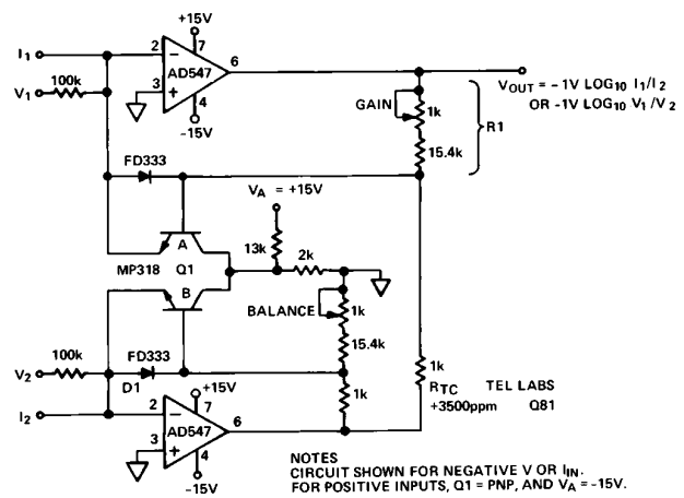
Figure 33. Log-Ratio Amplifier
