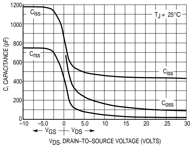
Figure 8. Capacitance Variation
