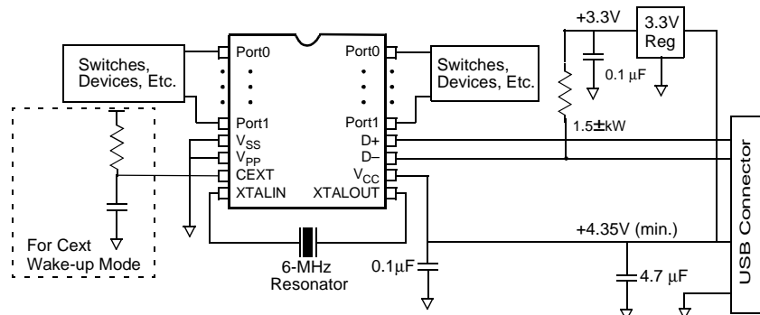
Figure 6-28. Application Showing 1.5-kΩ ±5% Pull-Up Resistor
