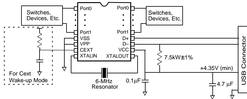
Figure 6-27. Application Showing 7.5kΩ ±1% Pull-Up Resistor
