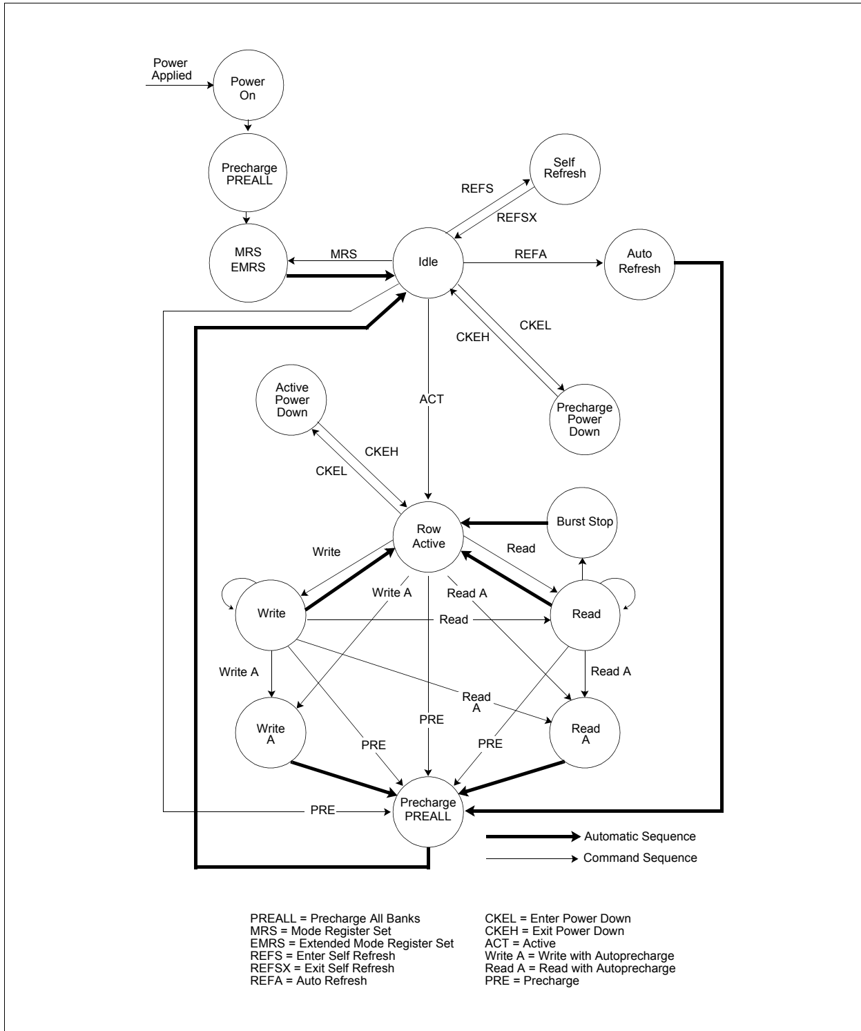
Figure 33 Simplified State Diagram
