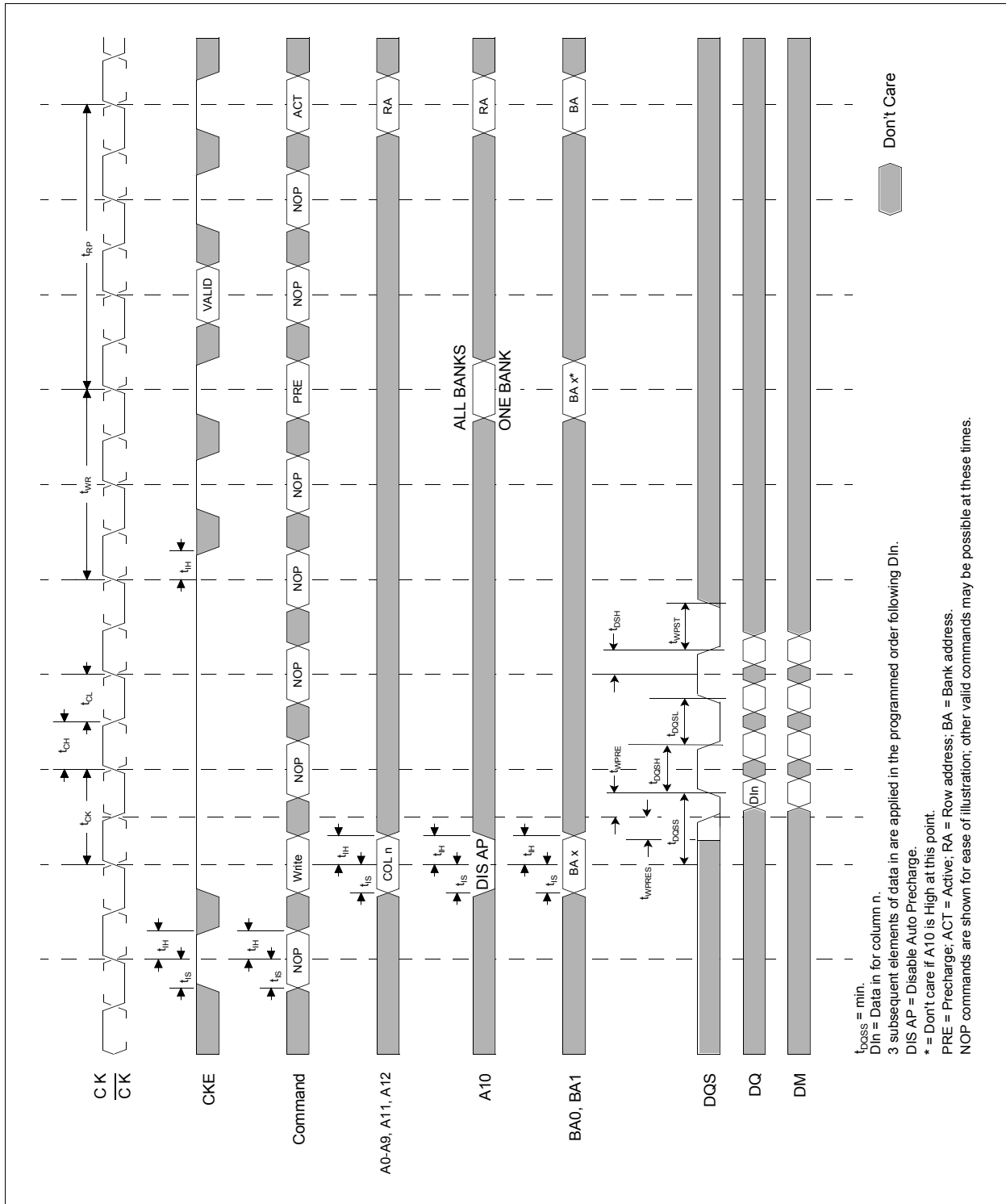
Figure 48 Write without Auto Precharge (Burst Length = 4)
