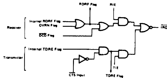
Figure 14 \overline{IRQ} Internal Circuit
